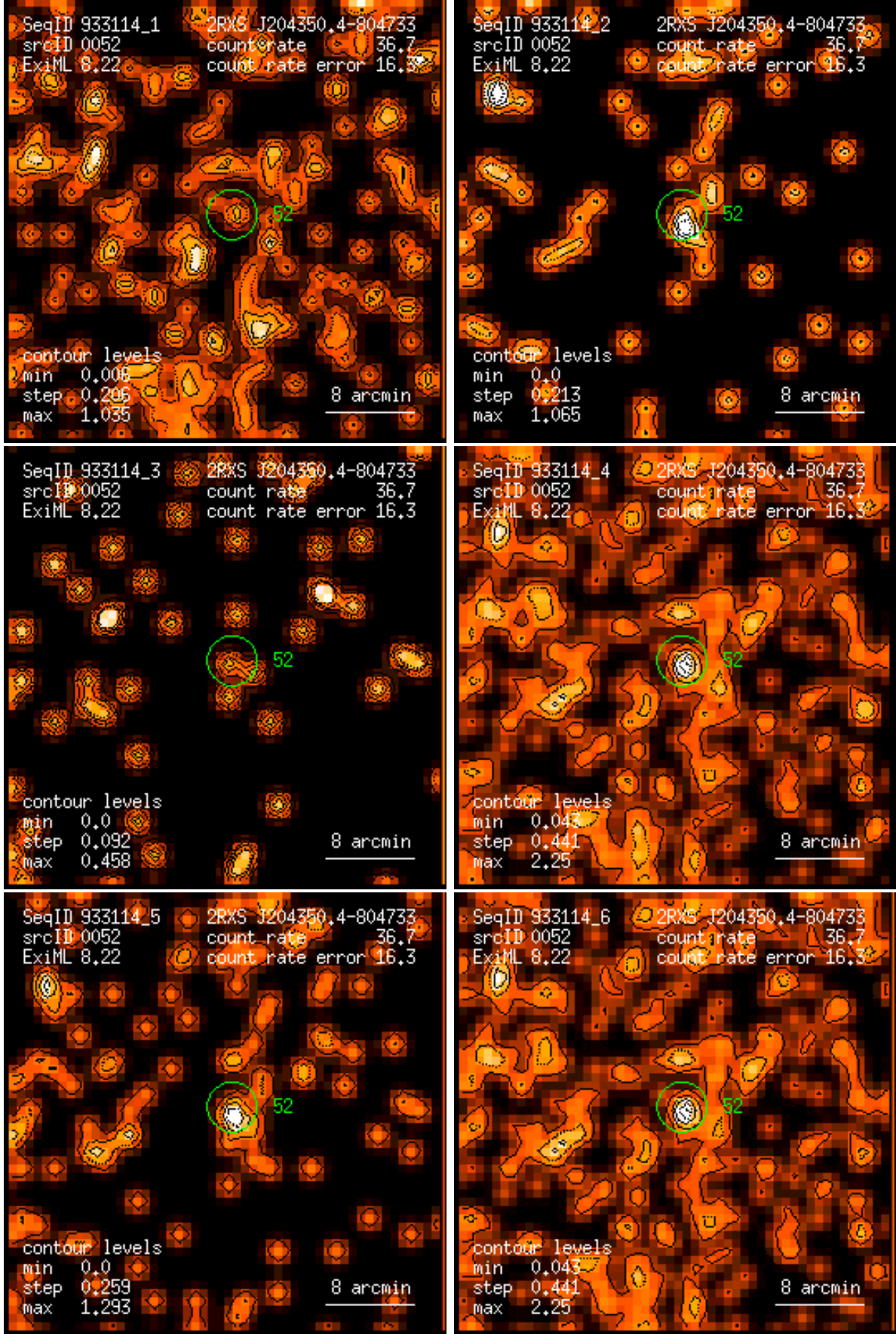
Figure 52: RASS 933114: detection 0052: band rate images, Gaussian filter: (1) PSPC channels 11 – 41, (2) 52 – 90, (3) 91 – 201, (4) 11 – 235, (5) 52 – 201, (6) 11 – 201. Broad band rates in counts/ks. Band rate contour levels in counts/ks/arcmin 2 .
