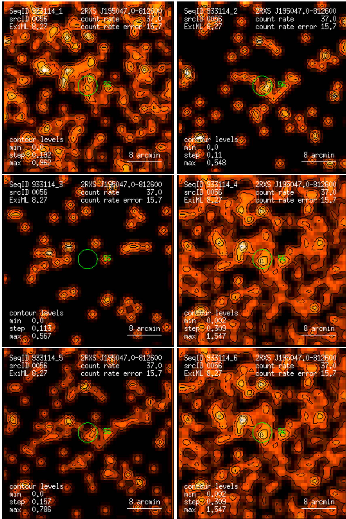
Figure 56: RASS 933114: detection 0056: band rate images, Gaussian filter: (1) PSPC channels 11 – 41, (2) 52 – 90, (3) 91 – 201, (4) 11 – 235, (5) 52 – 201, (6) 11 – 201. Broad band rates in counts/ks. Band rate contour levels in counts/ks/arcmin 2 .
