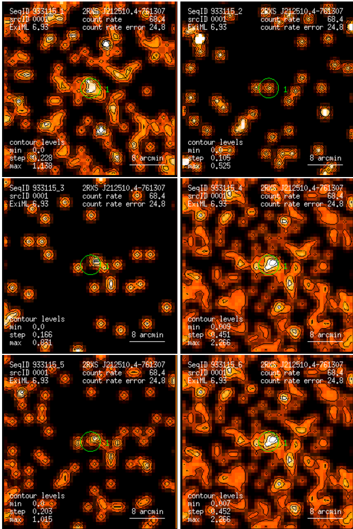
Figure 1: RASS 933115: detection 0001: band rate images, Gaussian filter: (1) PSPC channels 11 – 41, (2) 52 – 90, (3) 91 – 201, (4) 11 – 235, (5) 52 – 201, (6) 11 – 201. Broad band rates in counts/ks. Band rate contour levels in counts/ks/arcmin 2 .
