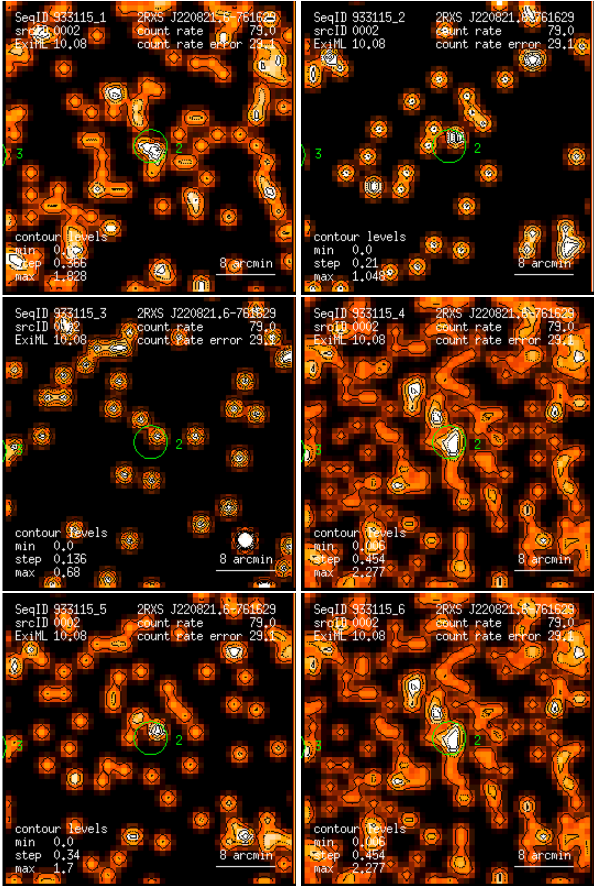
Figure 2: RASS 933115: detection 0002: band rate images, Gaussian filter: (1) PSPC channels 11 – 41, (2) 52 – 90, (3) 91 – 201, (4) 11 – 235, (5) 52 – 201, (6) 11 – 201. Broad band rates in counts/ks. Band rate contour levels in counts/ks/arcmin 2 .
