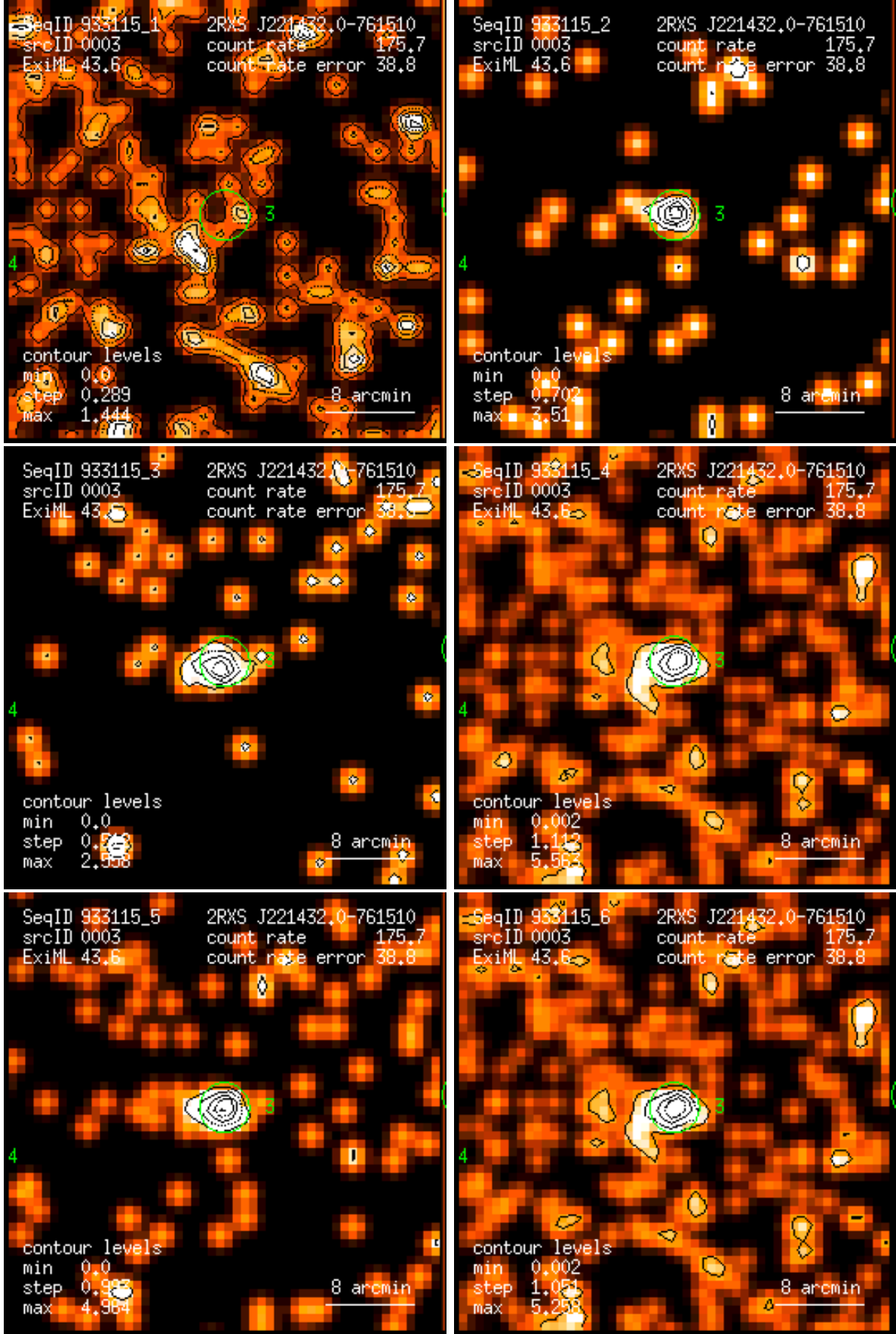
Figure 3: RASS 933115: detection 0003: band rate images, Gaussian filter: (1) PSPC channels 11 – 41, (2) 52 – 90, (3) 91 – 201, (4) 11 – 235, (5) 52 – 201, (6) 11 – 201. Broad band rates in counts/ks. Band rate contour levels in counts/ks/arcmin 2 .
