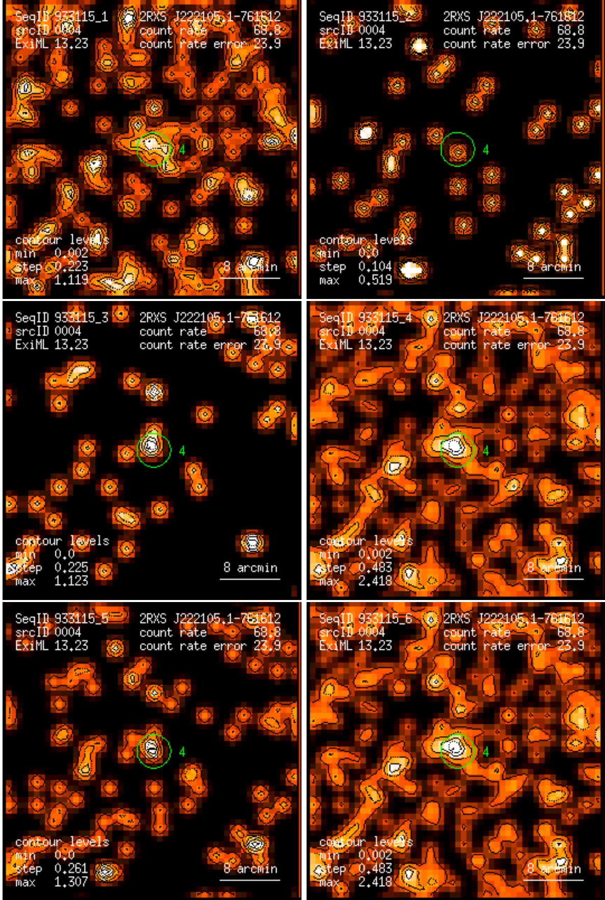
Figure 4: RASS 933115: detection 0004: band rate images, Gaussian filter: (1) PSPC channels 11 – 41, (2) 52 – 90, (3) 91 – 201, (4) 11 – 235, (5) 52 – 201, (6) 11 – 201. Broad band rates in counts/ks. Band rate contour levels in counts/ks/arcmin 2 .
