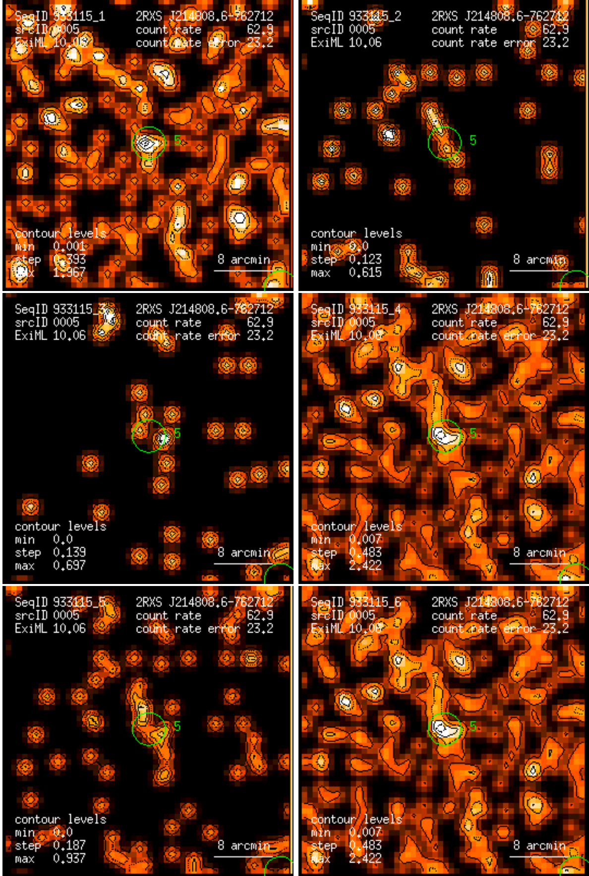
Figure 5: RASS 933115: detection 0005: band rate images, Gaussian filter: (1) PSPC channels 11 – 41, (2) 52 – 90, (3) 91 – 201, (4) 11 – 235, (5) 52 – 201, (6) 11 – 201. Broad band rates in counts/ks. Band rate contour levels in counts/ks/arcmin 2 .
