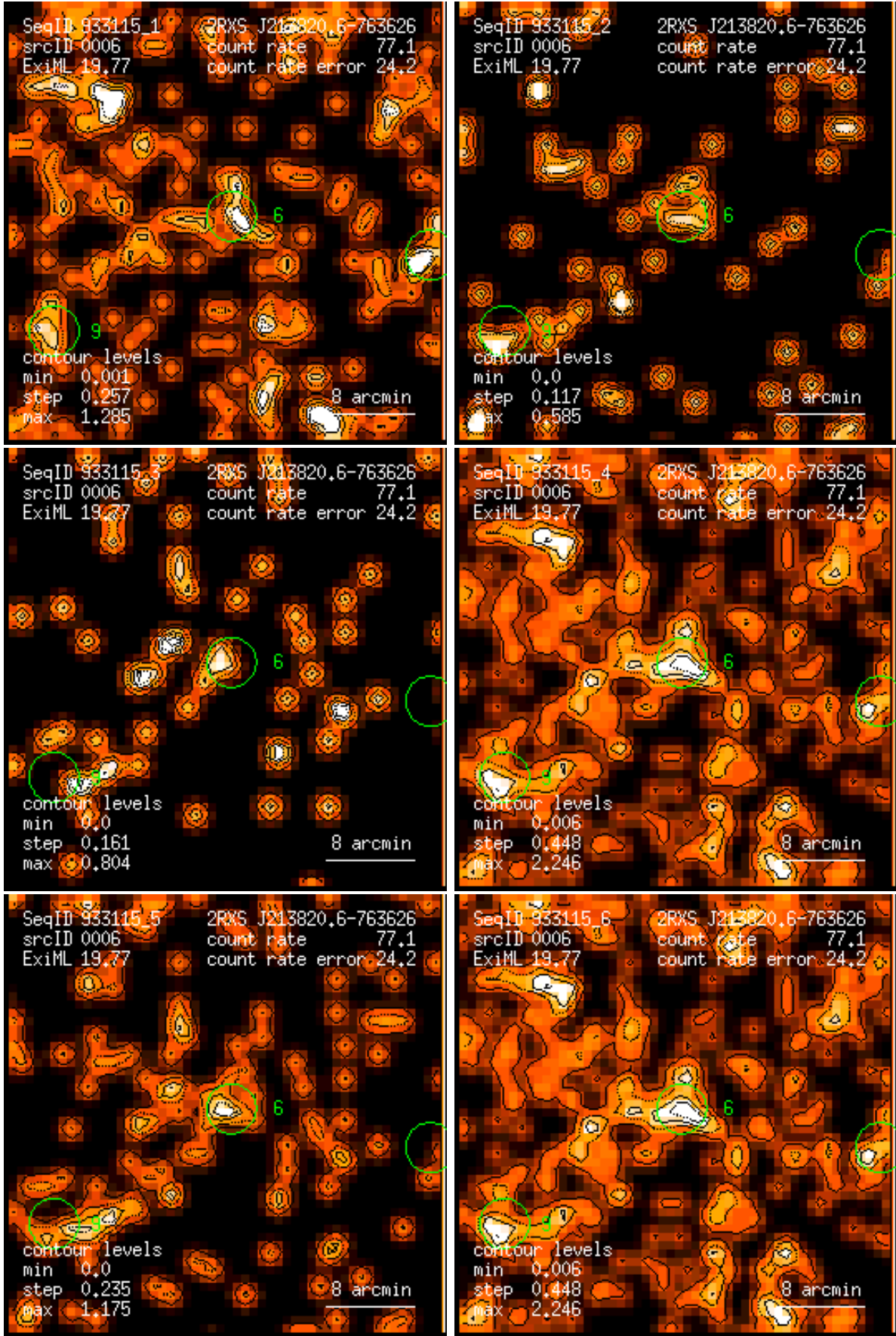
Figure 6: RASS 933115: detection 0006: band rate images, Gaussian filter: (1) PSPC channels 11 – 41, (2) 52 – 90, (3) 91 – 201, (4) 11 – 235, (5) 52 – 201, (6) 11 – 201. Broad band rates in counts/ks. Band rate contour levels in counts/ks/arcmin 2 .
