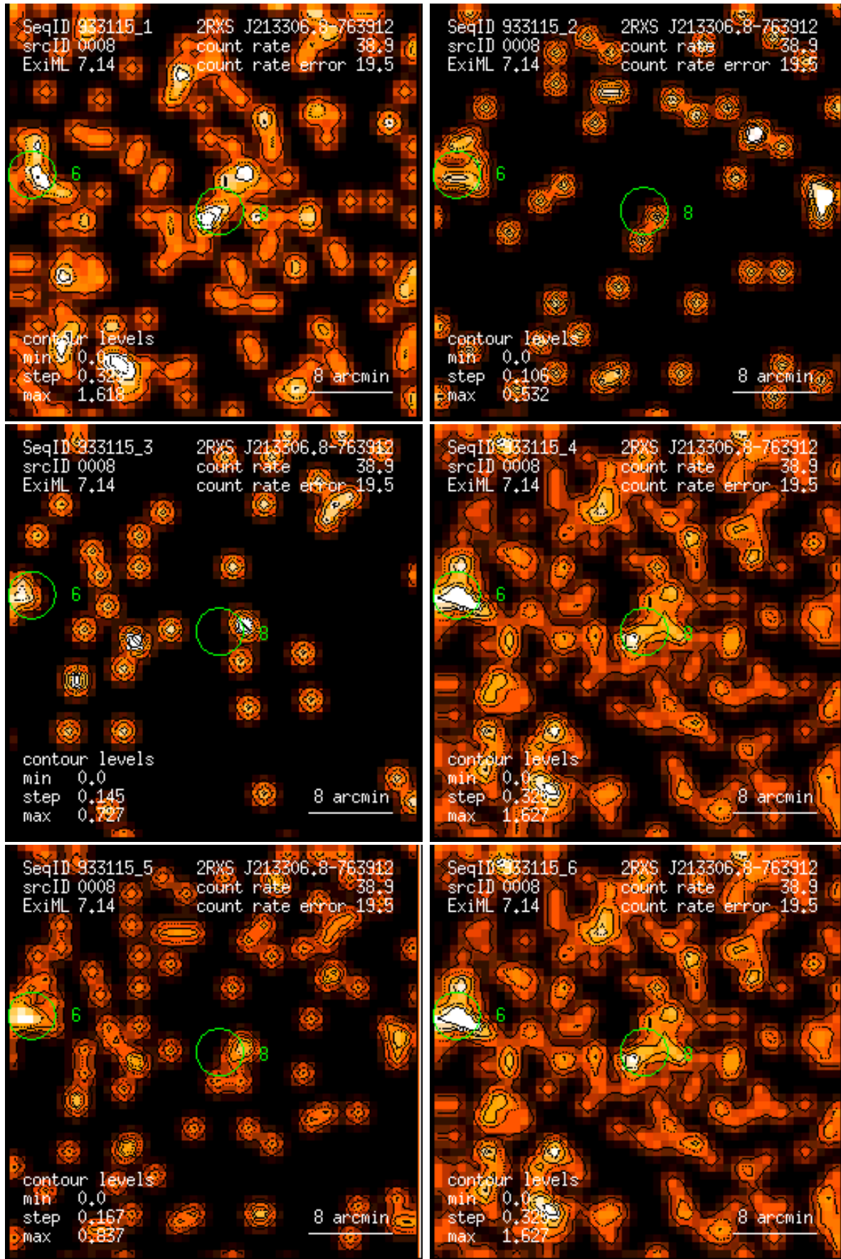
Figure 8: RASS 933115: detection 0008: band rate images, Gaussian filter: (1) PSPC channels 11 – 41, (2) 52 – 90, (3) 91 – 201, (4) 11 – 235, (5) 52 – 201, (6) 11 – 201. Broad band rates in counts/ks. Band rate contour levels in counts/ks/arcmin 2 .
