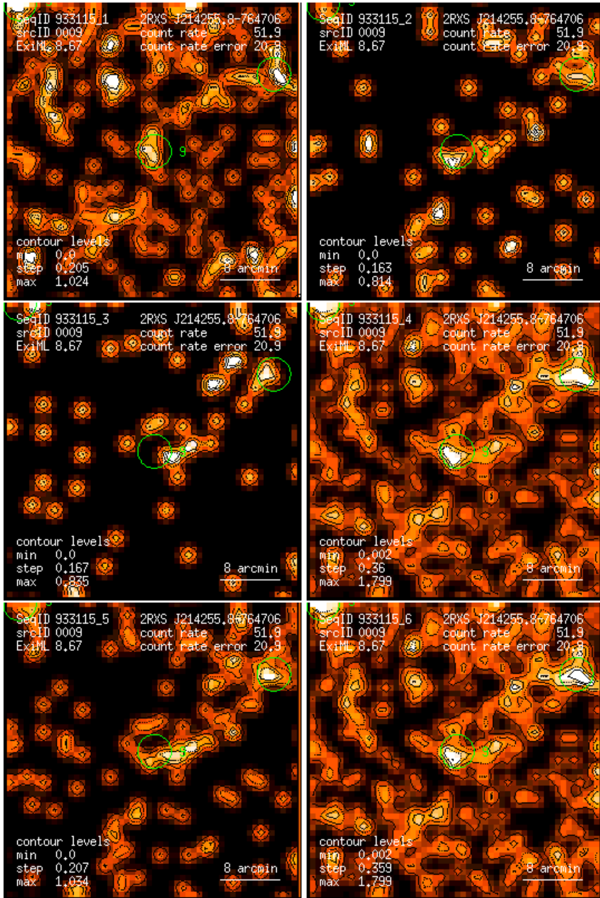
Figure 9: RASS 933115: detection 0009: band rate images, Gaussian filter: (1) PSPC channels 11 – 41, (2) 52 – 90, (3) 91 – 201, (4) 11 – 235, (5) 52 – 201, (6) 11 – 201. Broad band rates in counts/ks. Band rate contour levels in counts/ks/arcmin 2 .
