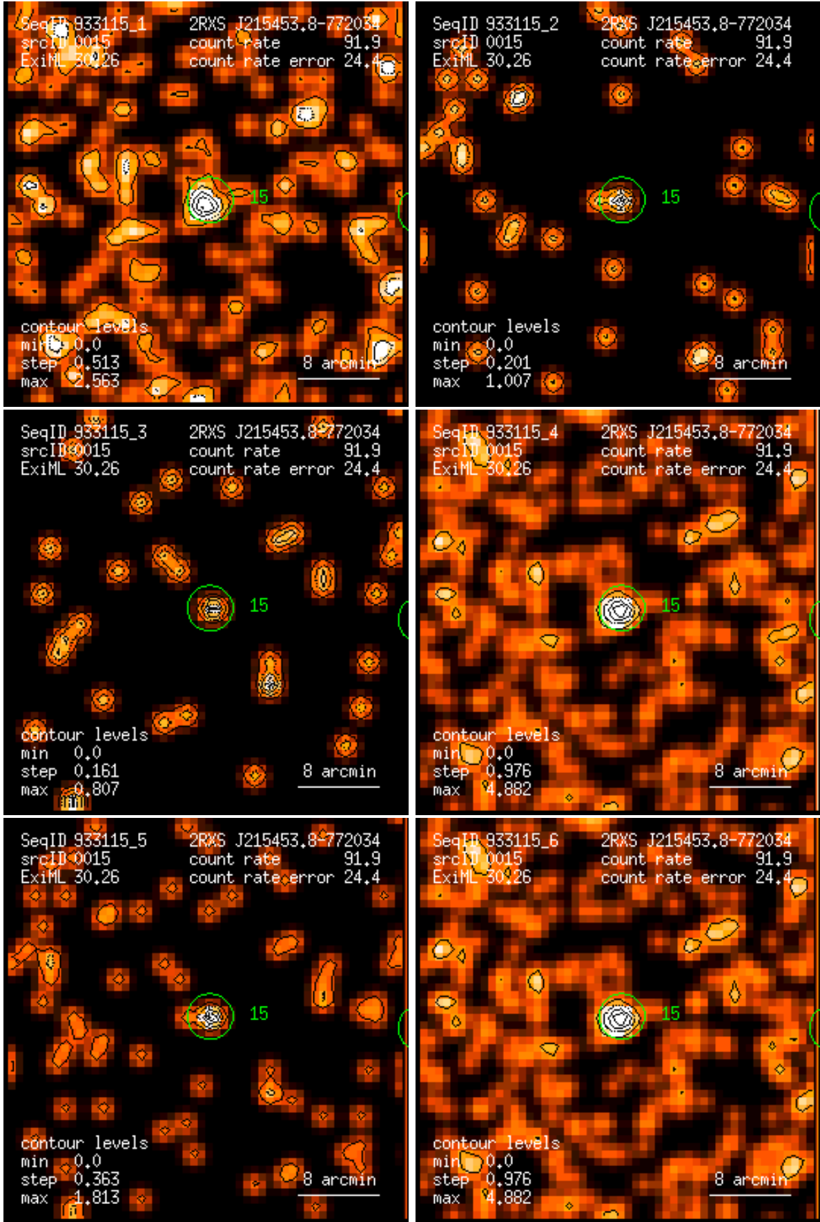
Figure 15: RASS 933115: detection 0015: band rate images, Gaussian filter: (1) PSPC channels 11 – 41, (2) 52 – 90, (3) 91 – 201, (4) 11 – 235, (5) 52 – 201, (6) 11 – 201. Broad band rates in counts/ks. Band rate contour levels in counts/ks/arcmin 2 .
