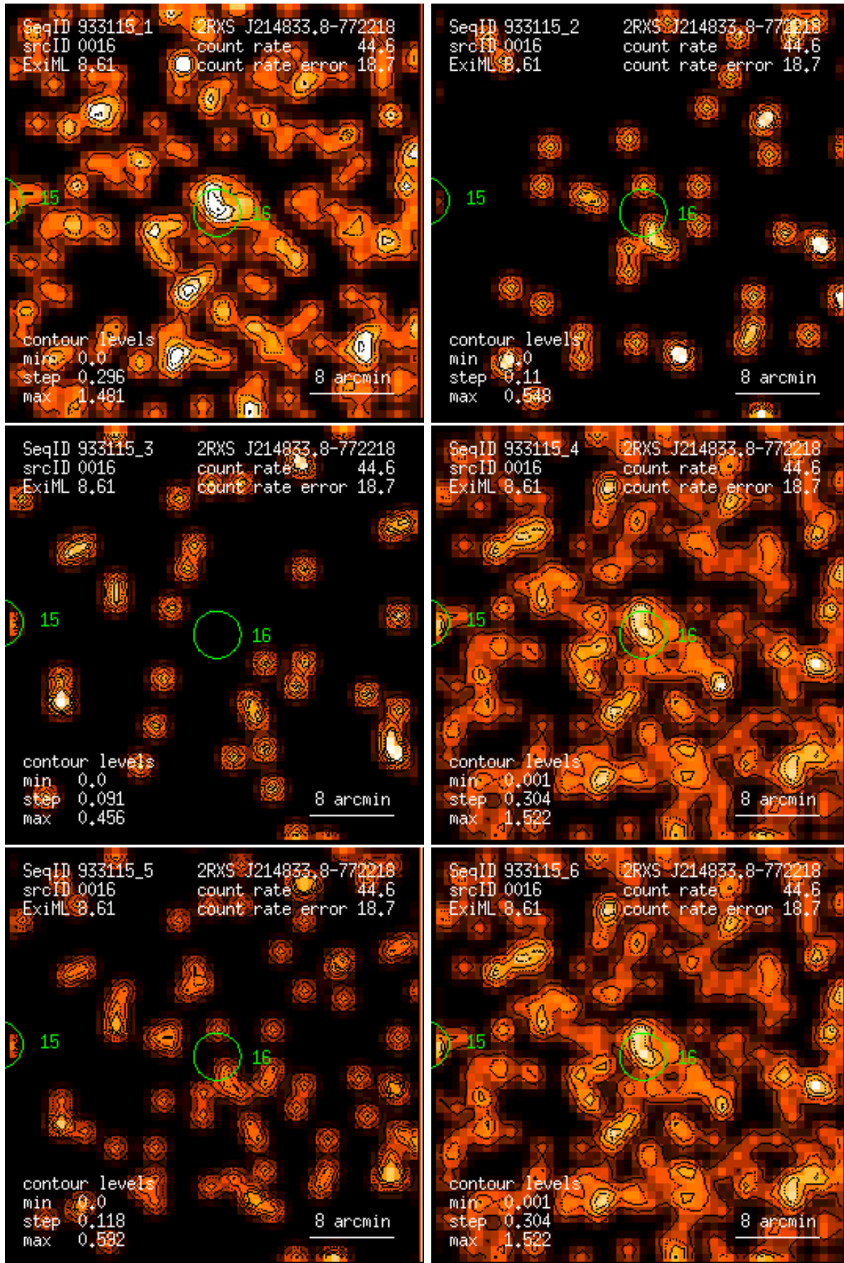
Figure 16: RASS 933115: detection 0016: band rate images, Gaussian filter: (1) PSPC channels 11 – 41, (2) 52 – 90, (3) 91 – 201, (4) 11 – 235, (5) 52 – 201, (6) 11 – 201. Broad band rates in counts/ks. Band rate contour levels in counts/ks/arcmin 2 .
