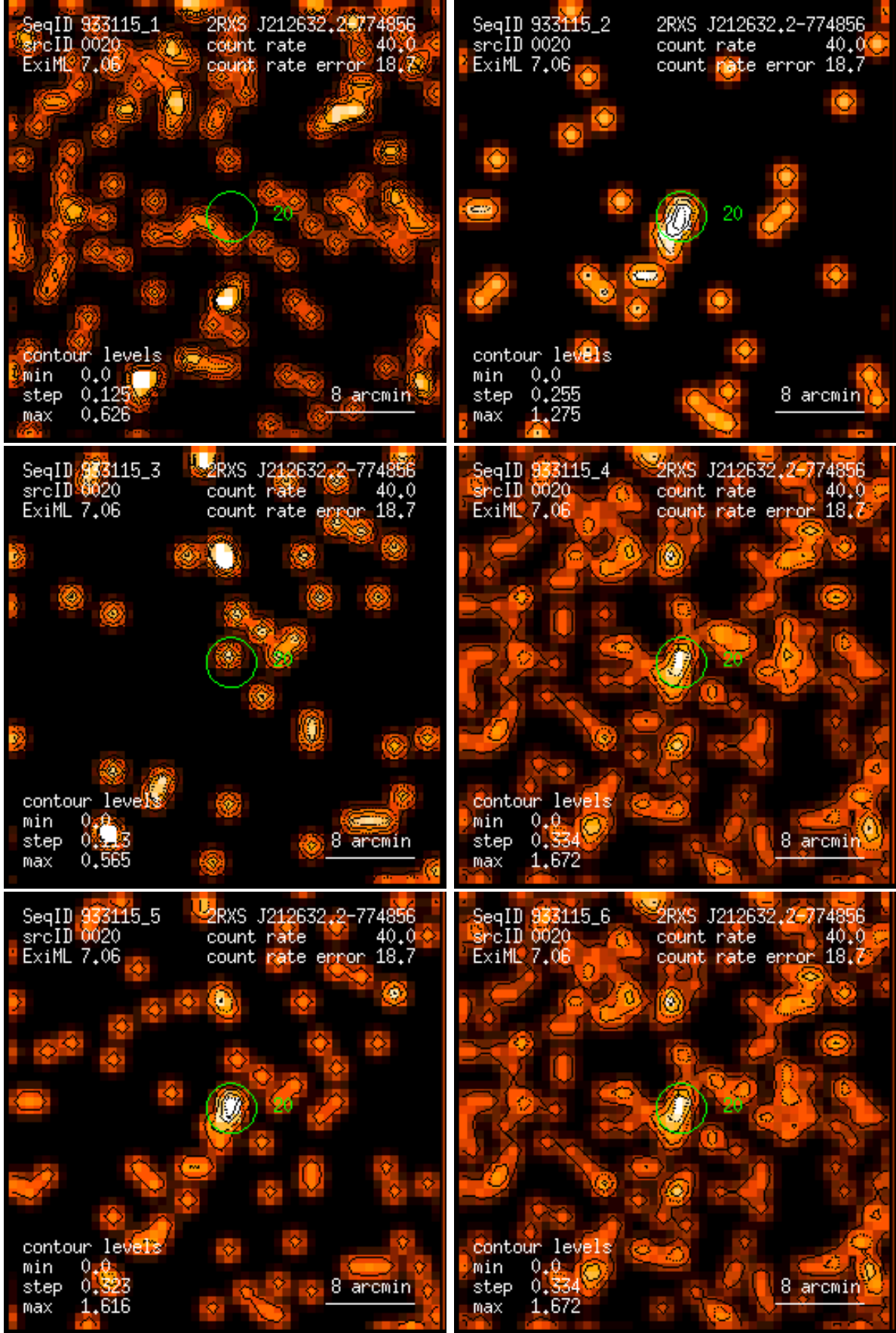
Figure 20: RASS 933115: detection 0020: band rate images, Gaussian filter: (1) PSPC channels 11 – 41, (2) 52 – 90, (3) 91 – 201, (4) 11 – 235, (5) 52 – 201, (6) 11 – 201. Broad band rates in counts/ks. Band rate contour levels in counts/ks/arcmin 2 .
