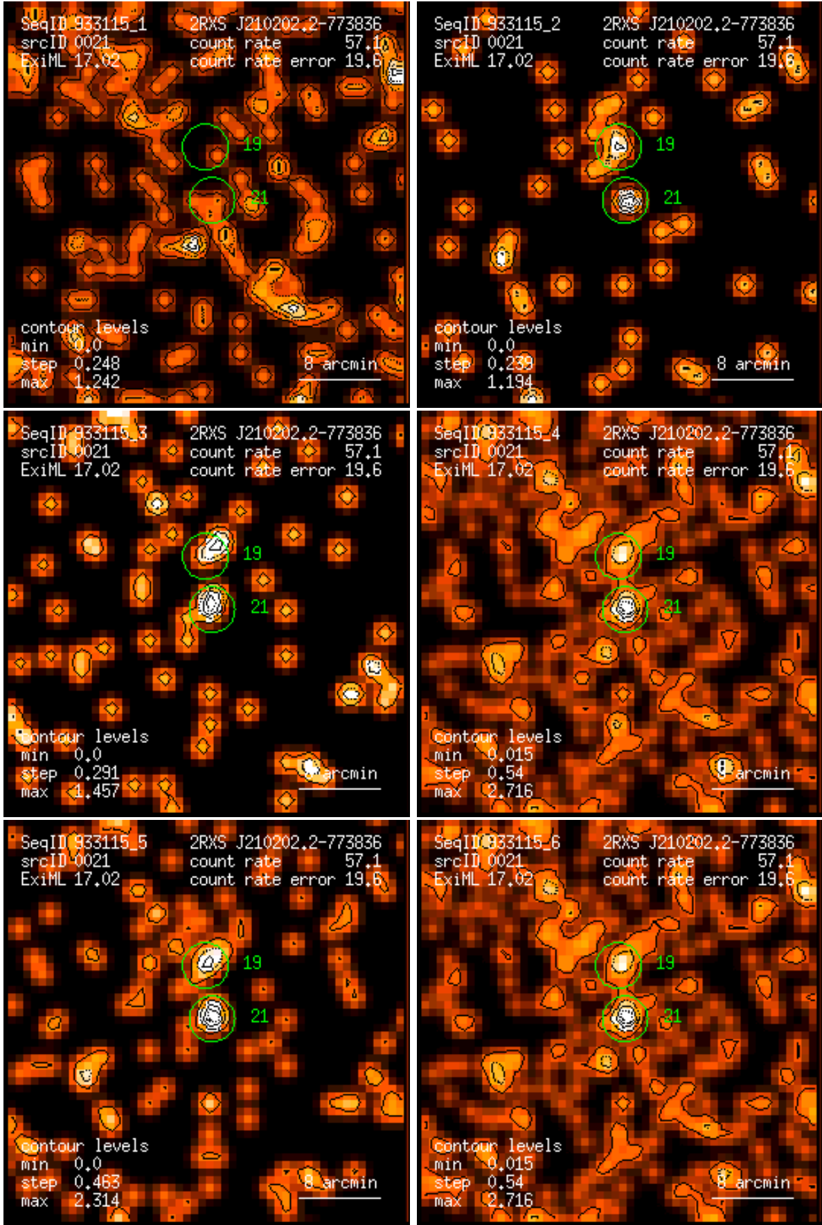
Figure 21: RASS 933115: detection 0021: band rate images, Gaussian filter: (1) PSPC channels 11 – 41, (2) 52 – 90, (3) 91 – 201, (4) 11 – 235, (5) 52 – 201, (6) 11 – 201. Broad band rates in counts/ks. Band rate contour levels in counts/ks/arcmin 2 .
