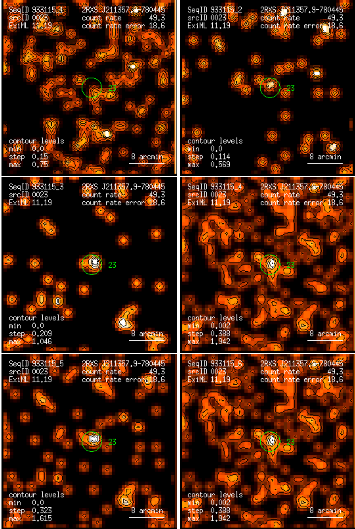
Figure 23: RASS 933115: detection 0023: band rate images, Gaussian filter: (1) PSPC channels 11 – 41, (2) 52 – 90, (3) 91 – 201, (4) 11 – 235, (5) 52 – 201, (6) 11 – 201. Broad band rates in counts/ks. Band rate contour levels in counts/ks/arcmin 2 .
