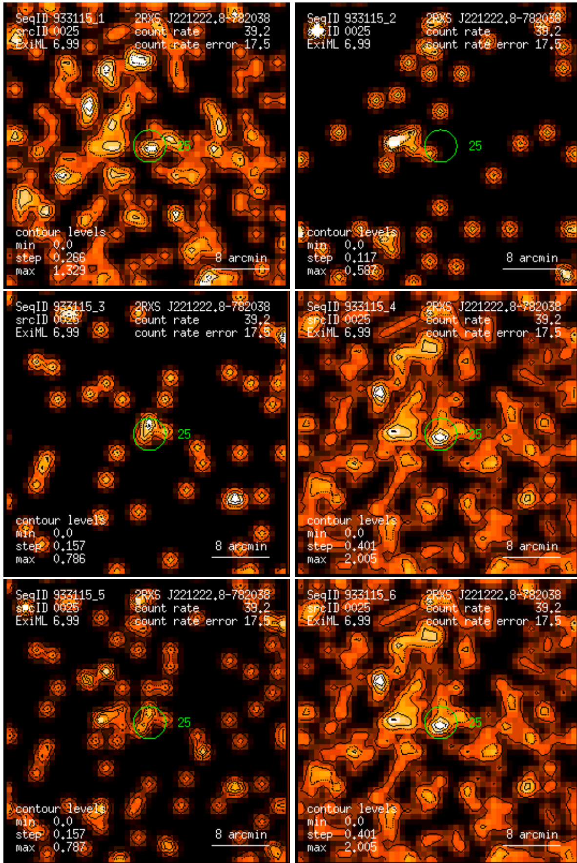
Figure 25: RASS 933115: detection 0025: band rate images, Gaussian filter: (1) PSPC channels 11 – 41, (2) 52 – 90, (3) 91 – 201, (4) 11 – 235, (5) 52 – 201, (6) 11 – 201. Broad band rates in counts/ks. Band rate contour levels in counts/ks/arcmin 2 .
