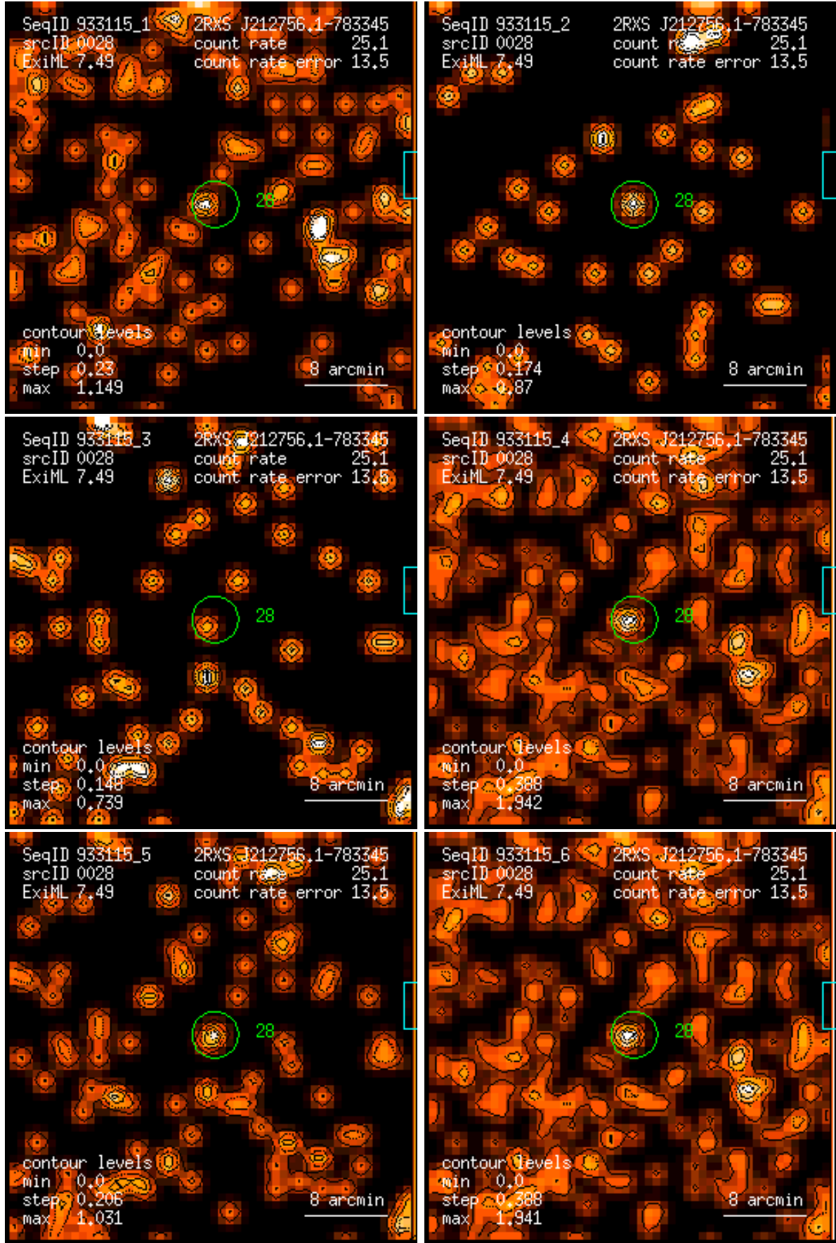
Figure 28: RASS 933115: detection 0028: band rate images, Gaussian filter: (1) PSPC channels 11 – 41, (2) 52 – 90, (3) 91 – 201, (4) 11 – 235, (5) 52 – 201, (6) 11 – 201. Broad band rates in counts/ks. Band rate contour levels in counts/ks/arcmin 2 .
