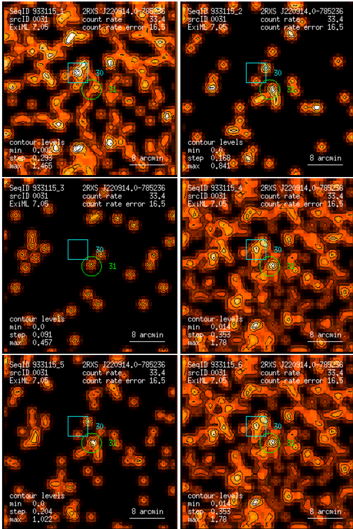
Figure 31: RASS 933115: detection 0031: band rate images, Gaussian filter: (1) PSPC channels 11 – 41, (2) 52 – 90, (3) 91 – 201, (4) 11 – 235, (5) 52 – 201, (6) 11 – 201. Broad band rates in counts/ks. Band rate contour levels in counts/ks/arcmin 2 .
