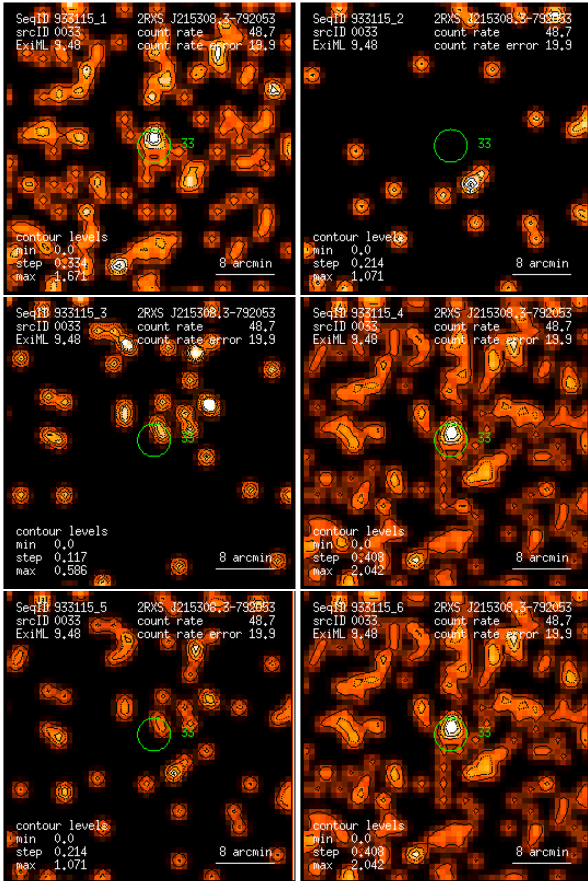
Figure 33: RASS 933115: detection 0033: band rate images, Gaussian filter: (1) PSPC channels 11 – 41, (2) 52 – 90, (3) 91 – 201, (4) 11 – 235, (5) 52 – 201, (6) 11 – 201. Broad band rates in counts/ks. Band rate contour levels in counts/ks/arcmin 2 .
