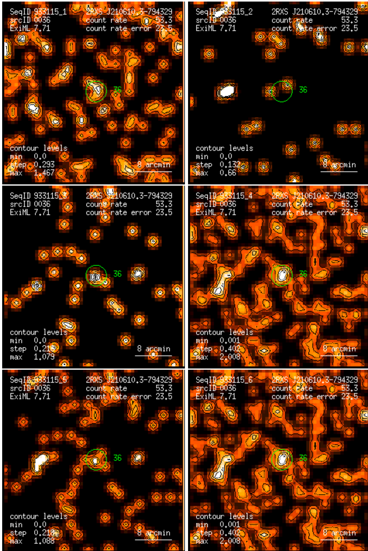
Figure 36: RASS 933115: detection 0036: band rate images, Gaussian filter: (1) PSPC channels 11 – 41, (2) 52 – 90, (3) 91 – 201, (4) 11 – 235, (5) 52 – 201, (6) 11 – 201. Broad band rates in counts/ks. Band rate contour levels in counts/ks/arcmin 2 .
