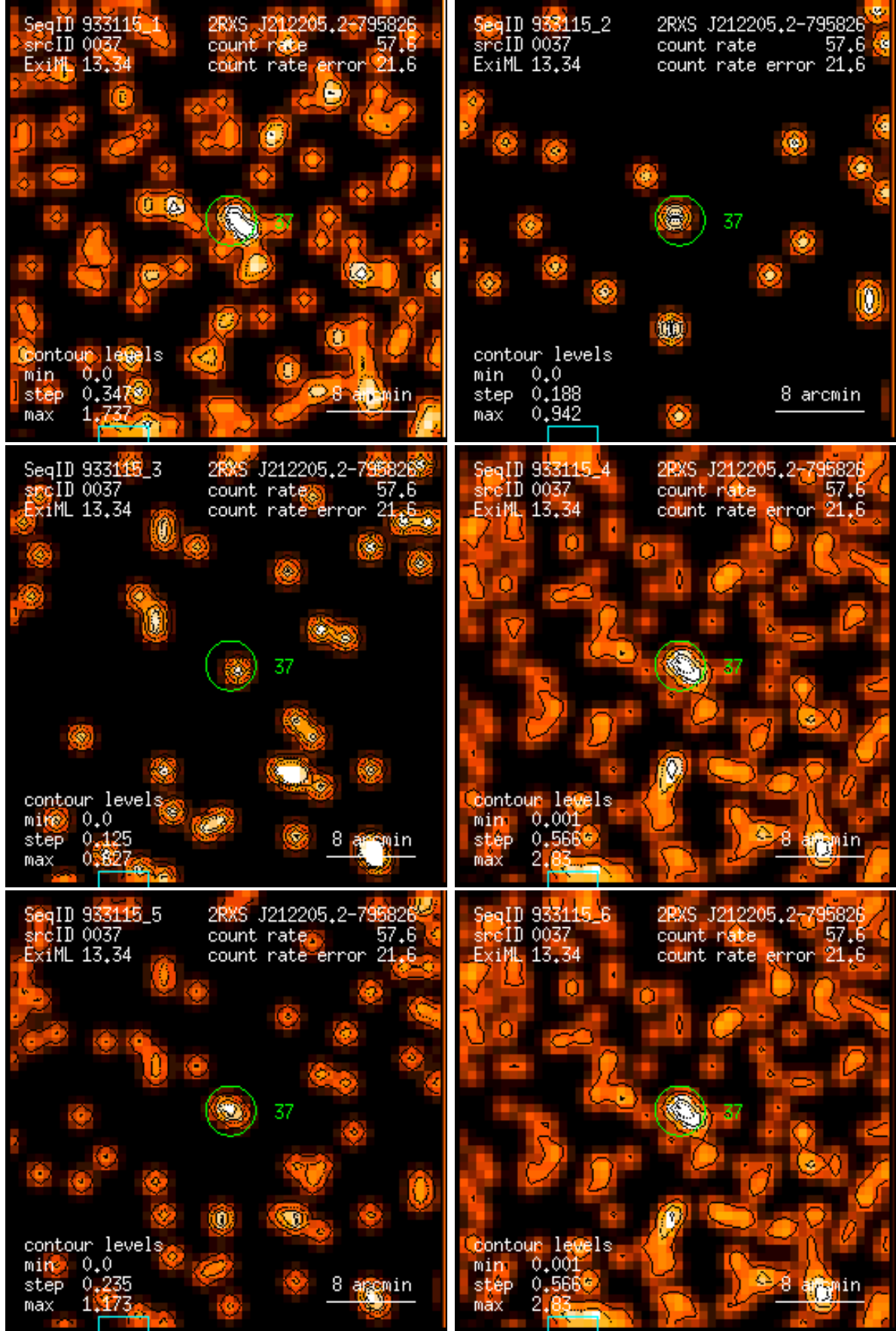
Figure 37: RASS 933115: detection 0037: band rate images, Gaussian filter: (1) PSPC channels 11 – 41, (2) 52 – 90, (3) 91 – 201, (4) 11 – 235, (5) 52 – 201, (6) 11 – 201. Broad band rates in counts/ks. Band rate contour levels in counts/ks/arcmin 2 .
