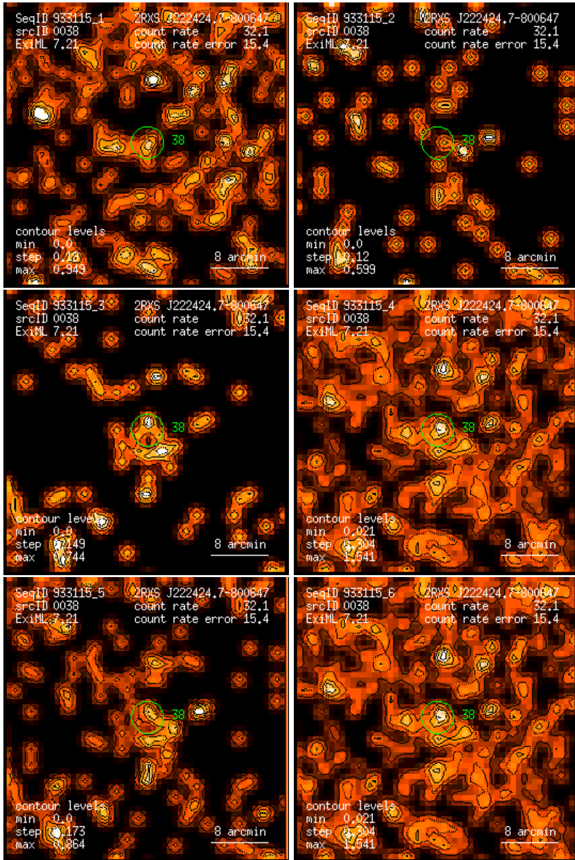
Figure 38: RASS 933115: detection 0038: band rate images, Gaussian filter: (1) PSPC channels 11 – 41, (2) 52 – 90, (3) 91 – 201, (4) 11 – 235, (5) 52 – 201, (6) 11 – 201. Broad band rates in counts/ks. Band rate contour levels in counts/ks/arcmin 2 .
