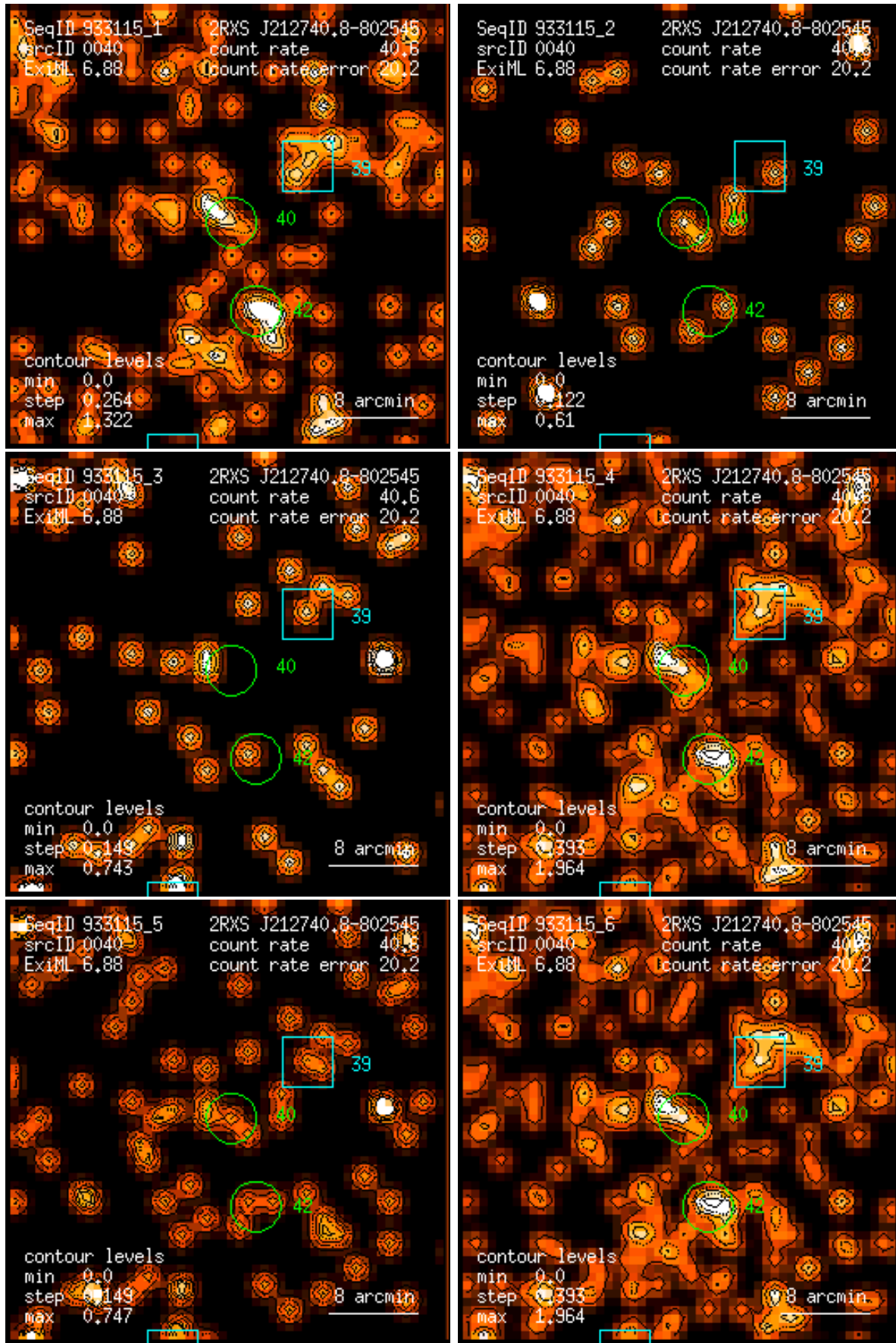
Figure 40: RASS 933115: detection 0040: band rate images, Gaussian filter: (1) PSPC channels 11 – 41, (2) 52 – 90, (3) 91 – 201, (4) 11 – 235, (5) 52 – 201, (6) 11 – 201. Broad band rates in counts/ks. Band rate contour levels in counts/ks/arcmin 2 .
