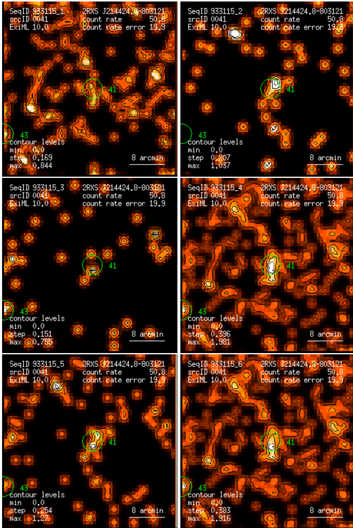
Figure 41: RASS 933115: detection 0041: band rate images, Gaussian filter: (1) PSPC channels 11 – 41, (2) 52 – 90, (3) 91 – 201, (4) 11 – 235, (5) 52 – 201, (6) 11 – 201. Broad band rates in counts/ks. Band rate contour levels in counts/ks/arcmin 2 .
