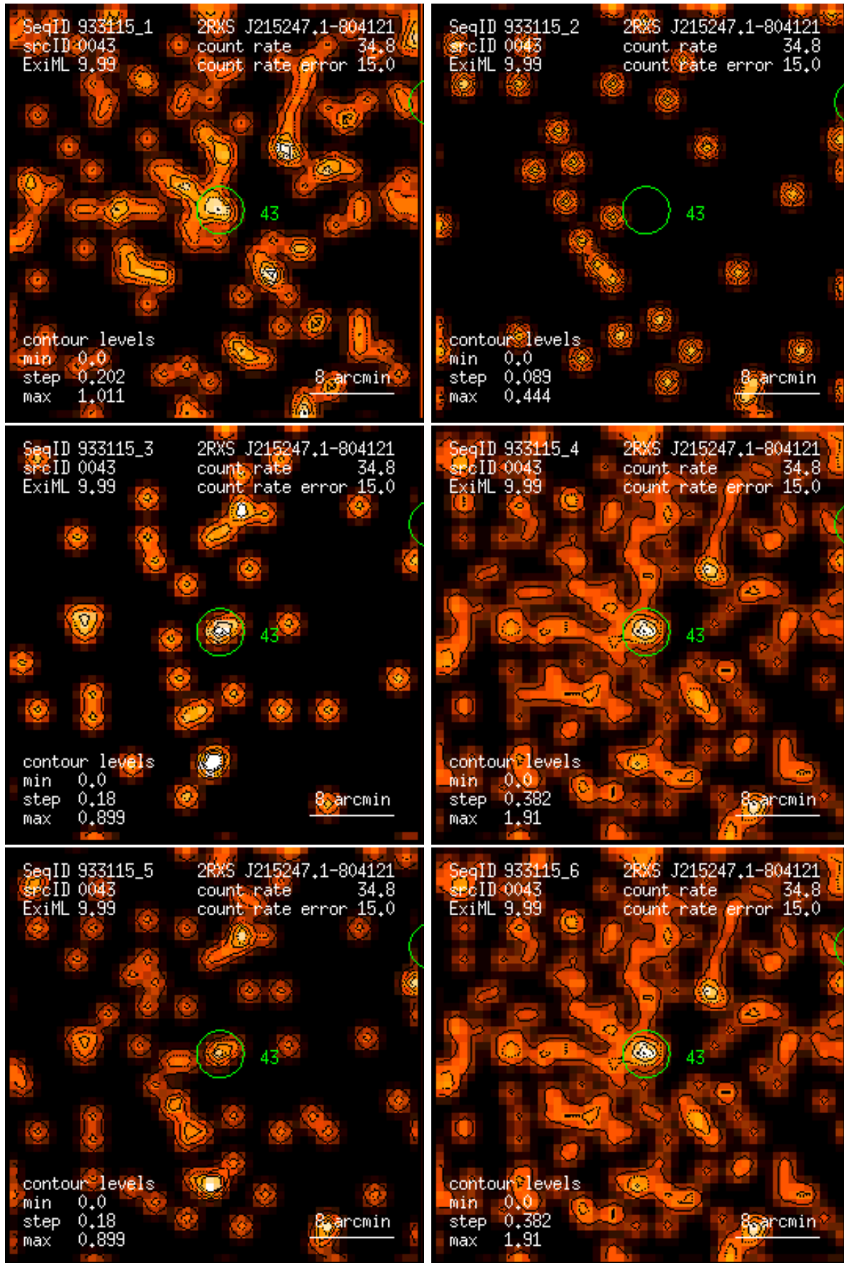
Figure 43: RASS 933115: detection 0043: band rate images, Gaussian filter: (1) PSPC channels 11 – 41, (2) 52 – 90, (3) 91 – 201, (4) 11 – 235, (5) 52 – 201, (6) 11 – 201. Broad band rates in counts/ks. Band rate contour levels in counts/ks/arcmin 2 .
