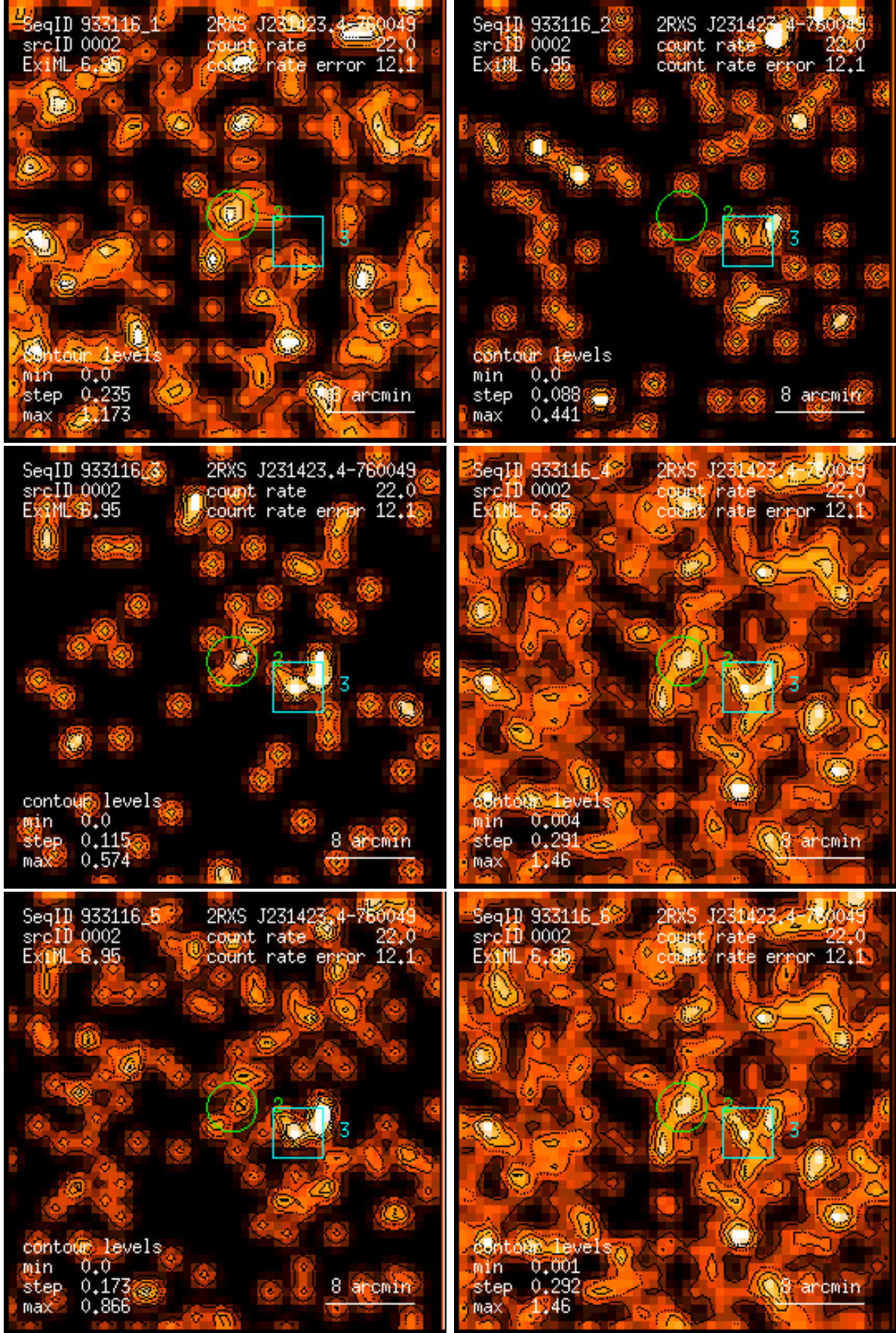
Figure 2: RASS 933116: detection 0002: band rate images, Gaussian filter: (1) PSPC channels 11 – 41, (2) 52 – 90, (3) 91 – 201, (4) 11 – 235, (5) 52 – 201, (6) 11 – 201. Broad band rates in counts/ks. Band rate contour levels in counts/ks/arcmin 2 .
