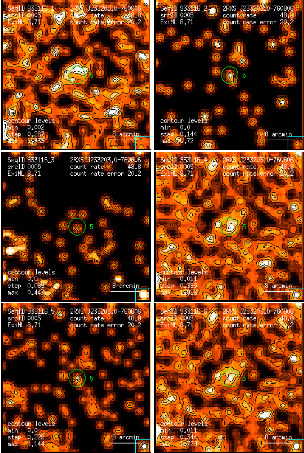
Figure 5: RASS 933116: detection 0005: band rate images, Gaussian filter: (1) PSPC channels 11 – 41, (2) 52 – 90, (3) 91 – 201, (4) 11 – 235, (5) 52 – 201, (6) 11 – 201. Broad band rates in counts/ks. Band rate contour levels in counts/ks/arcmin 2 .
