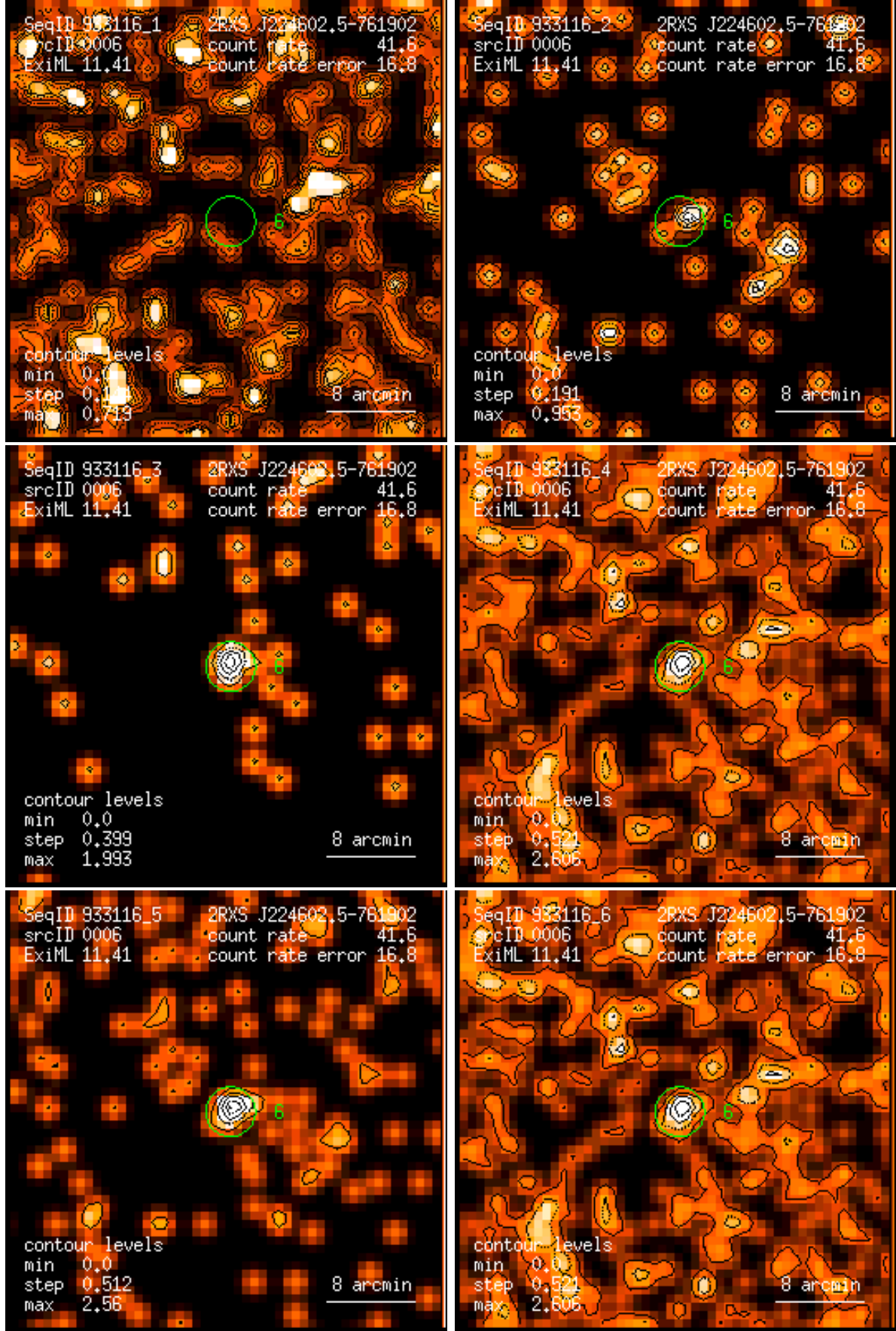
Figure 6: RASS 933116: detection 0006: band rate images, Gaussian filter: (1) PSPC channels 11 – 41, (2) 52 – 90, (3) 91 – 201, (4) 11 – 235, (5) 52 – 201, (6) 11 – 201. Broad band rates in counts/ks. Band rate contour levels in counts/ks/arcmin 2 .
