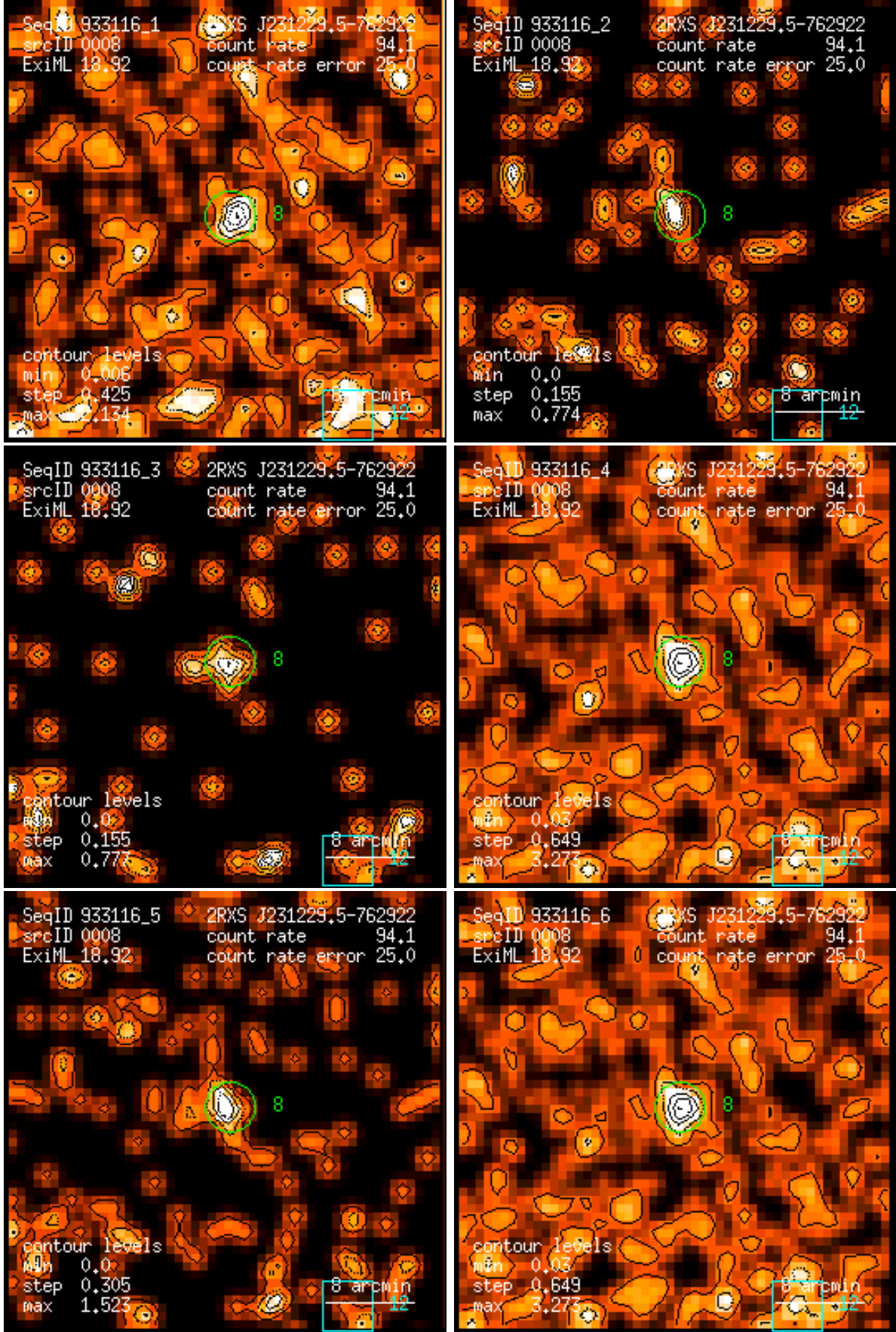
Figure 8: RASS 933116: detection 0008: band rate images, Gaussian filter: (1) PSPC channels 11 – 41, (2) 52 – 90, (3) 91 – 201, (4) 11 – 235, (5) 52 – 201, (6) 11 – 201. Broad band rates in counts/ks. Band rate contour levels in counts/ks/arcmin 2 .
