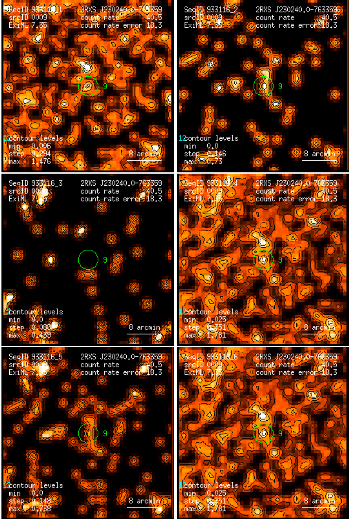
Figure 9: RASS 933116: detection 0009: band rate images, Gaussian filter: (1) PSPC channels 11 – 41, (2) 52 – 90, (3) 91 – 201, (4) 11 – 235, (5) 52 – 201, (6) 11 – 201. Broad band rates in counts/ks. Band rate contour levels in counts/ks/arcmin 2 .
