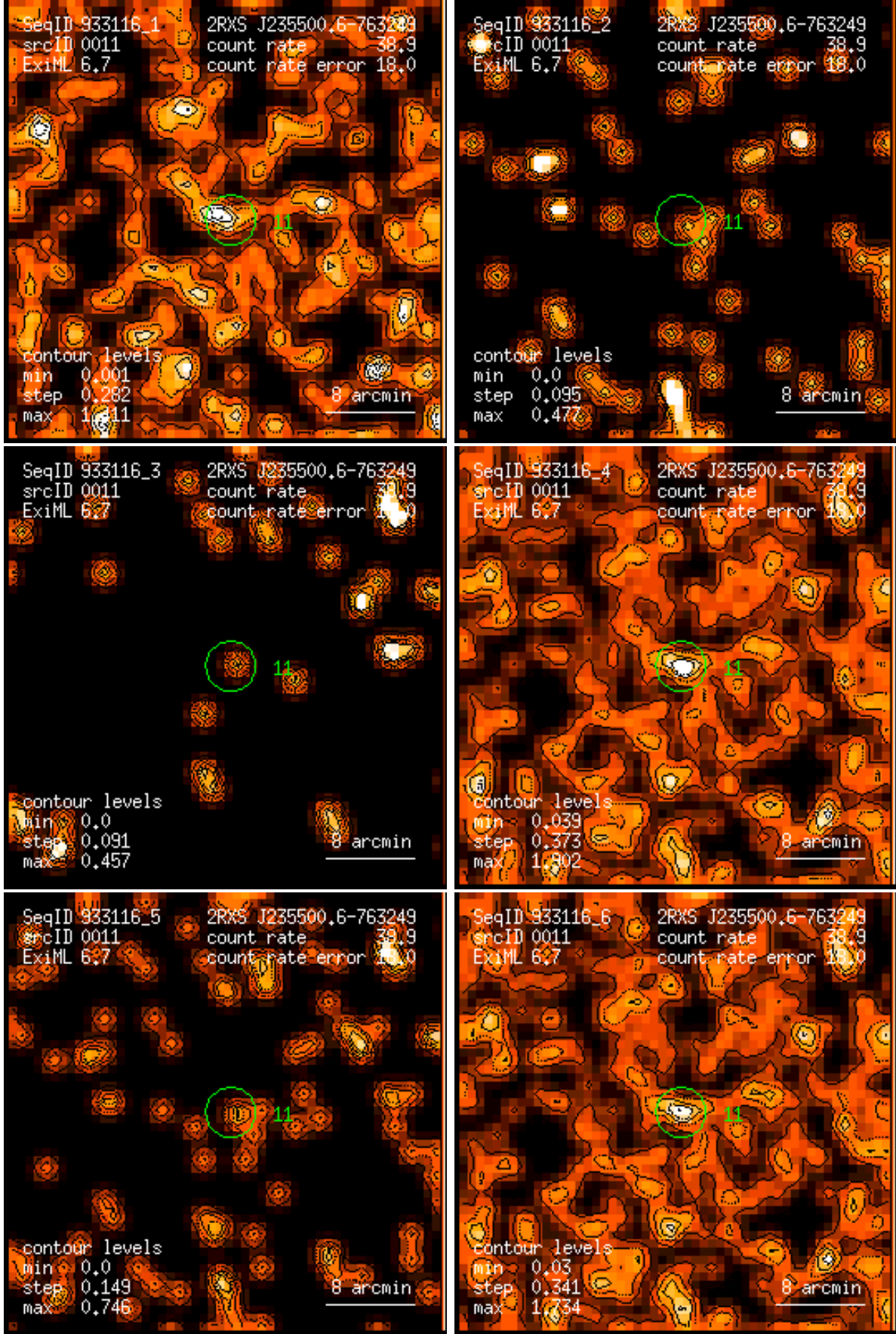
Figure 11: RASS 933116: detection 0011: band rate images, Gaussian filter: (1) PSPC channels 11 – 41, (2) 52 – 90, (3) 91 – 201, (4) 11 – 235, (5) 52 – 201, (6) 11 – 201. Broad band rates in counts/ks. Band rate contour levels in counts/ks/arcmin 2 .
