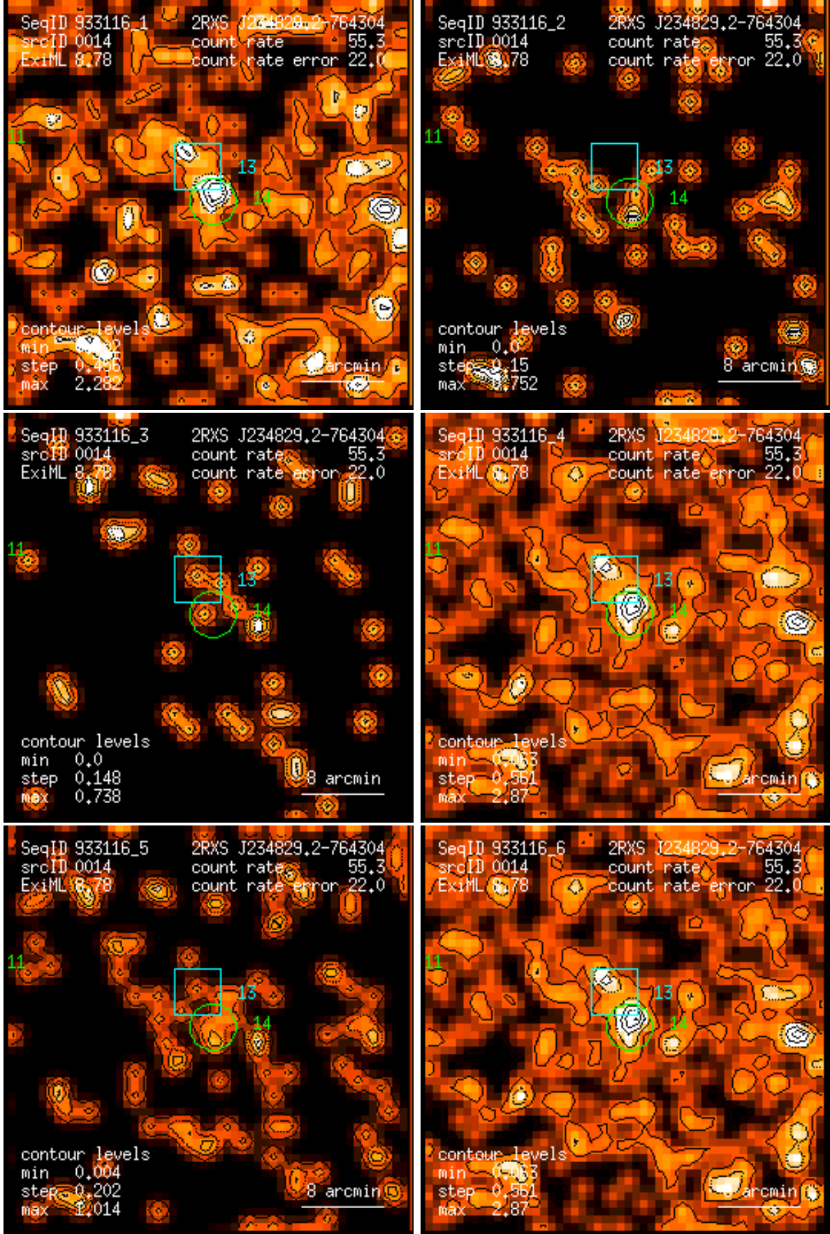
Figure 14: RASS 933116: detection 0014: band rate images, Gaussian filter: (1) PSPC channels 11 – 41, (2) 52 – 90, (3) 91 – 201, (4) 11 – 235, (5) 52 – 201, (6) 11 – 201. Broad band rates in counts/ks. Band rate contour levels in counts/ks/arcmin 2 .
