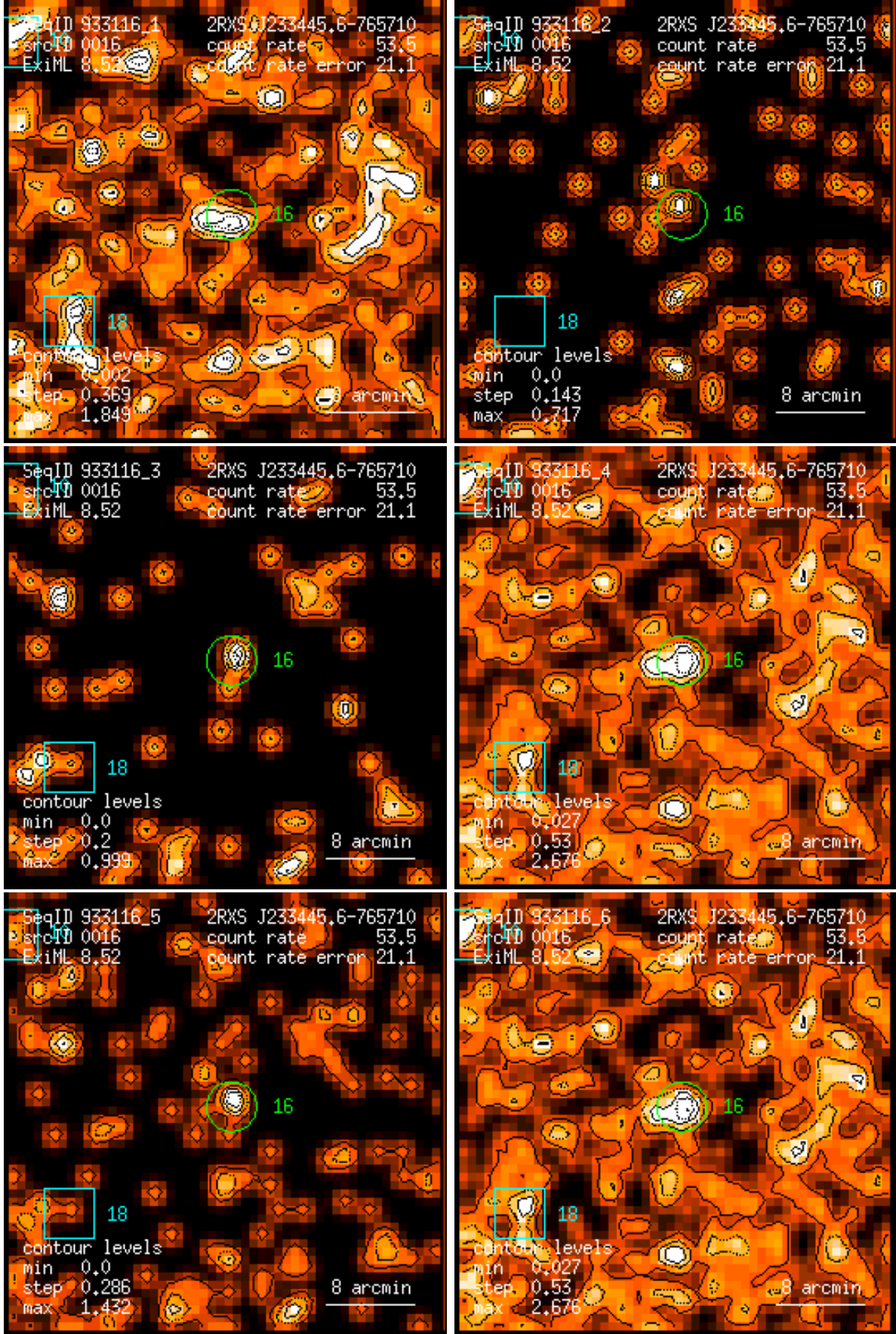
Figure 16: RASS 933116: detection 0016: band rate images, Gaussian filter: (1) PSPC channels 11 – 41, (2) 52 – 90, (3) 91 – 201, (4) 11 – 235, (5) 52 – 201, (6) 11 – 201. Broad band rates in counts/ks. Band rate contour levels in counts/ks/arcmin 2 .
