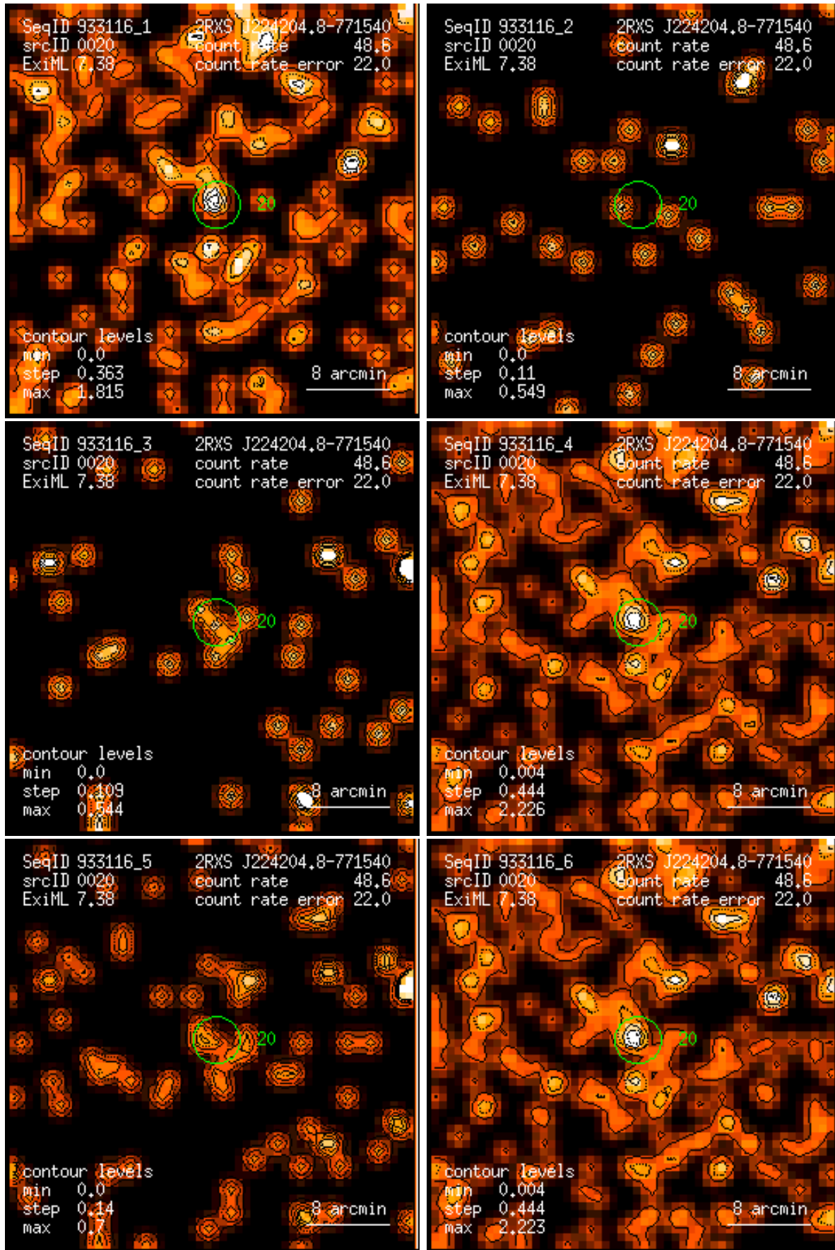
Figure 20: RASS 933116: detection 0020: band rate images, Gaussian filter: (1) PSPC channels 11 – 41, (2) 52 – 90, (3) 91 – 201, (4) 11 – 235, (5) 52 – 201, (6) 11 – 201. Broad band rates in counts/ks. Band rate contour levels in counts/ks/arcmin 2 .
