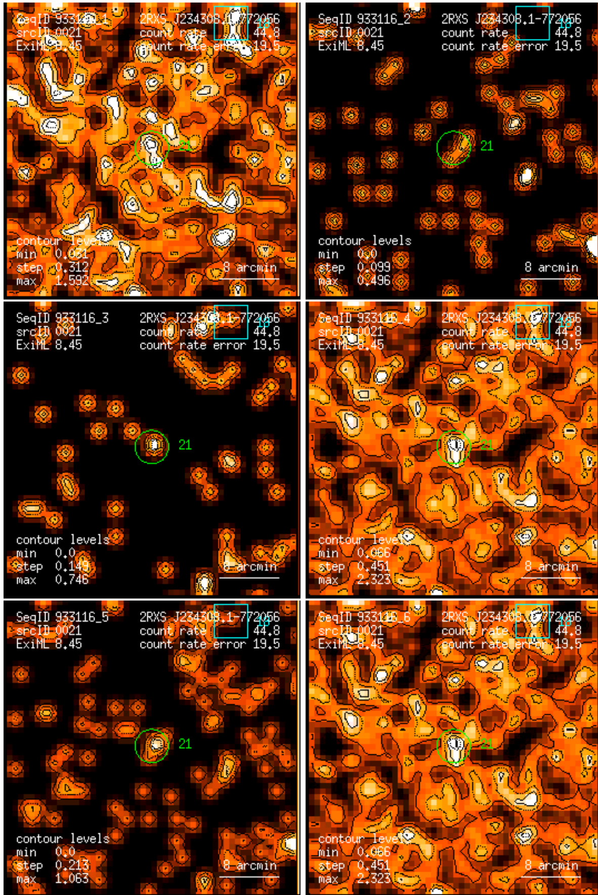
Figure 21: RASS 933116: detection 0021: band rate images, Gaussian filter: (1) PSPC channels 11 – 41, (2) 52 – 90, (3) 91 – 201, (4) 11 – 235, (5) 52 – 201, (6) 11 – 201. Broad band rates in counts/ks. Band rate contour levels in counts/ks/arcmin 2 .
