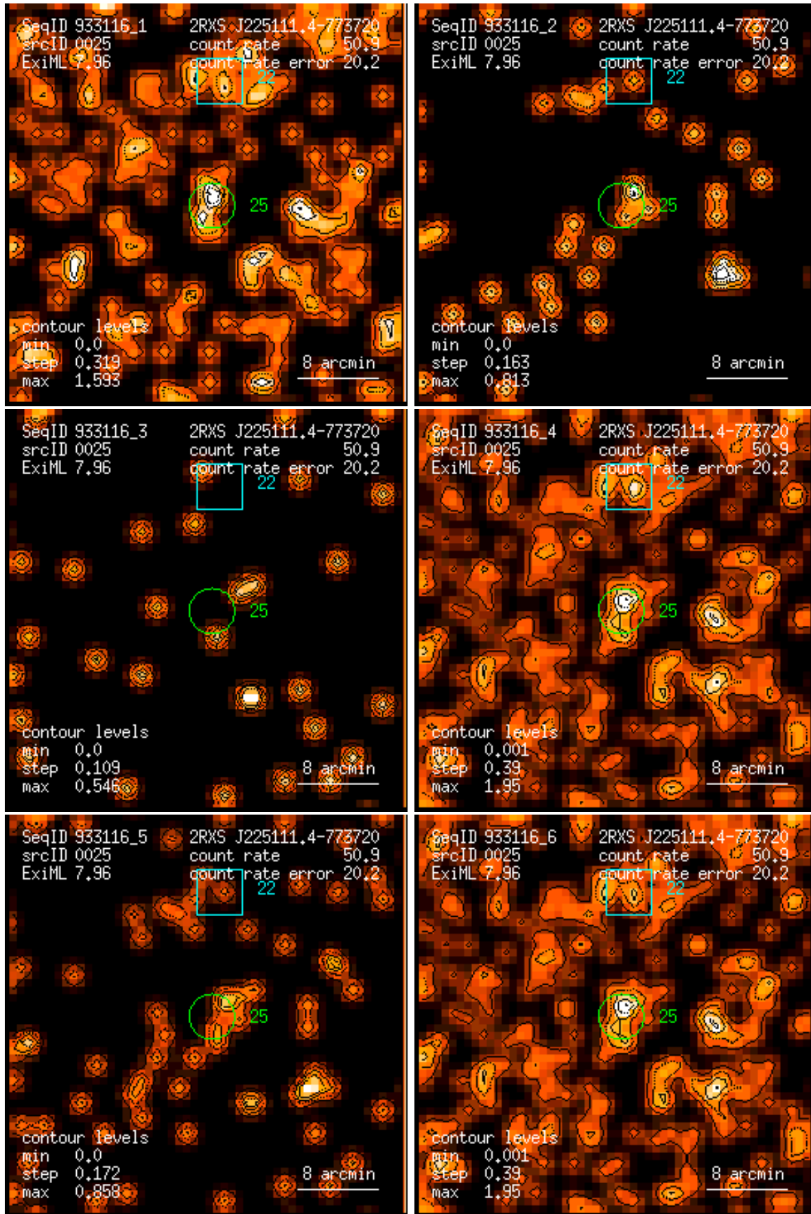
Figure 25: RASS 933116: detection 0025: band rate images, Gaussian filter: (1) PSPC channels 11 – 41, (2) 52 – 90, (3) 91 – 201, (4) 11 – 235, (5) 52 – 201, (6) 11 – 201. Broad band rates in counts/ks. Band rate contour levels in counts/ks/arcmin 2 .
