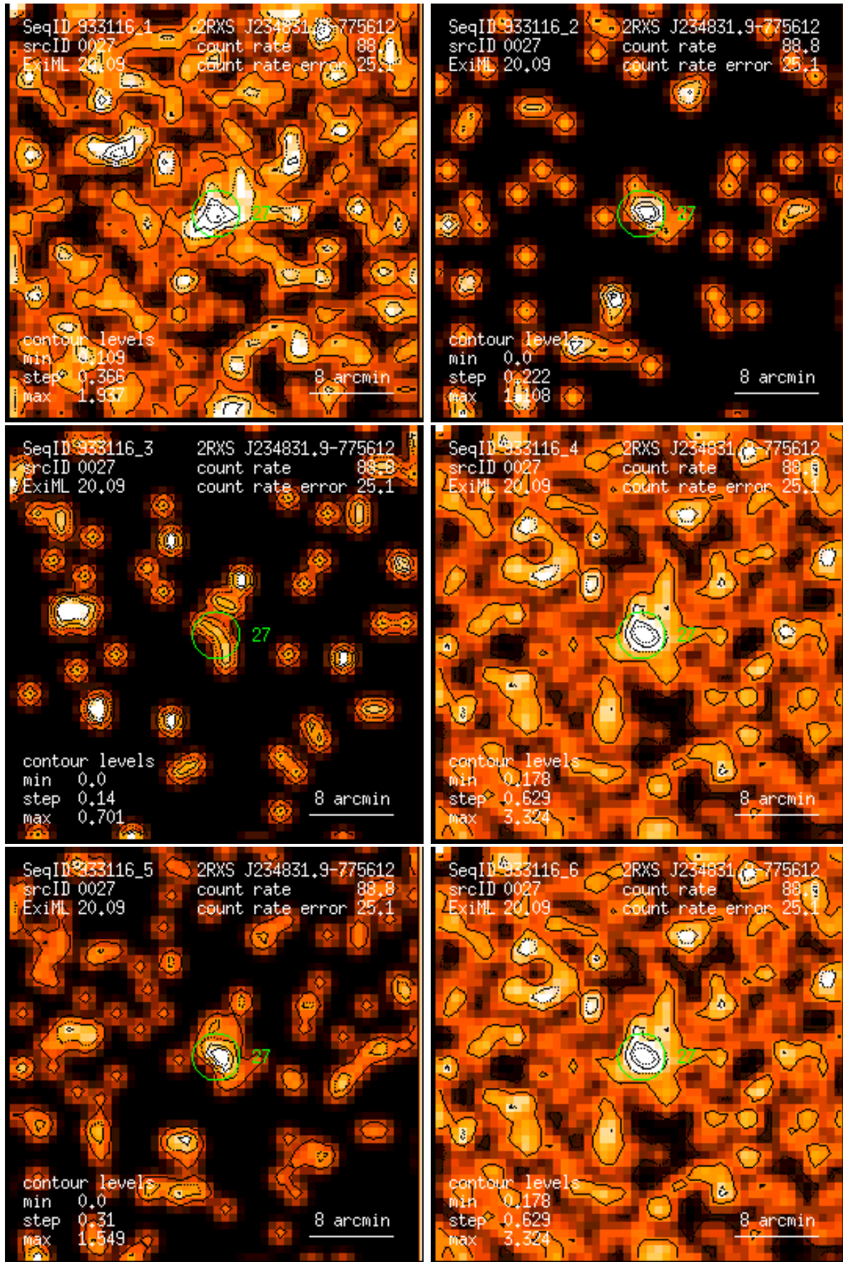
Figure 27: RASS 933116: detection 0027: band rate images, Gaussian filter: (1) PSPC channels 11 – 41, (2) 52 – 90, (3) 91 – 201, (4) 11 – 235, (5) 52 – 201, (6) 11 – 201. Broad band rates in counts/ks. Band rate contour levels in counts/ks/arcmin 2 .
