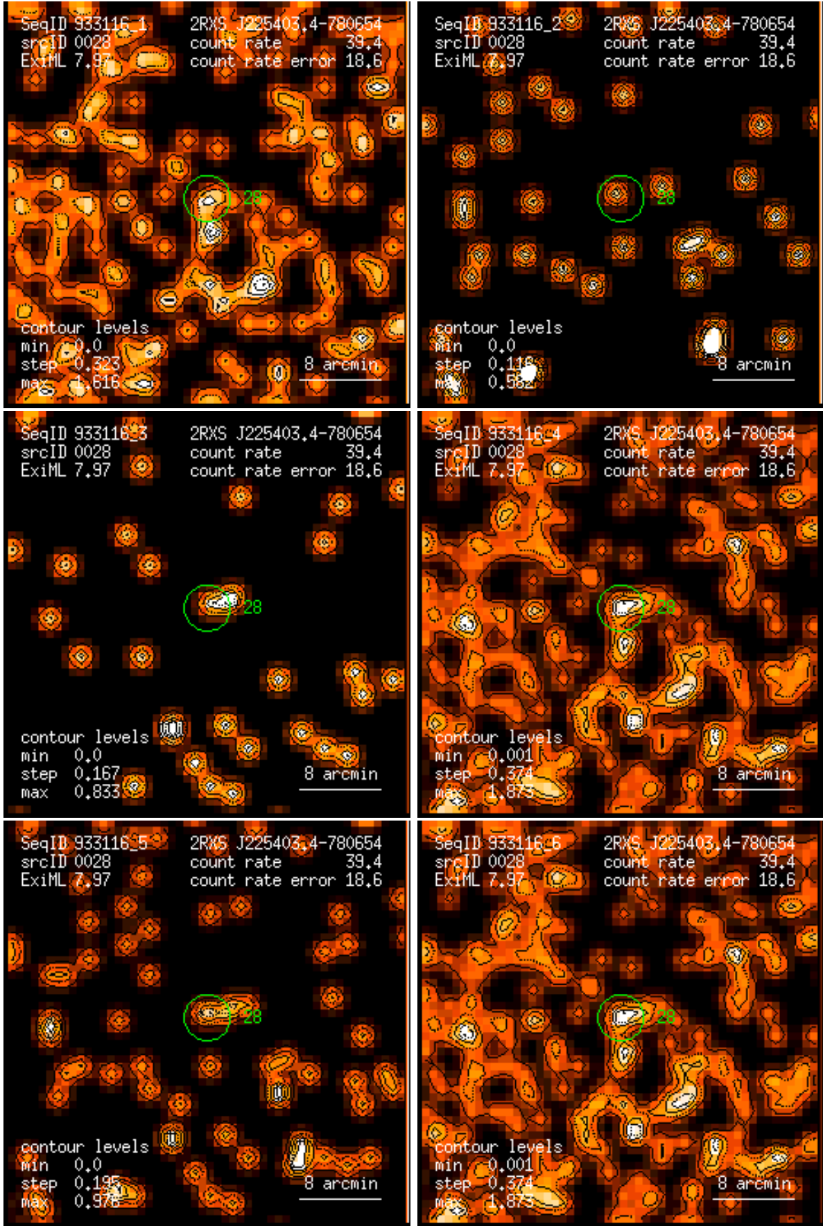
Figure 28: RASS 933116: detection 0028: band rate images, Gaussian filter: (1) PSPC channels 11 – 41, (2) 52 – 90, (3) 91 – 201, (4) 11 – 235, (5) 52 – 201, (6) 11 – 201. Broad band rates in counts/ks. Band rate contour levels in counts/ks/arcmin 2 .
