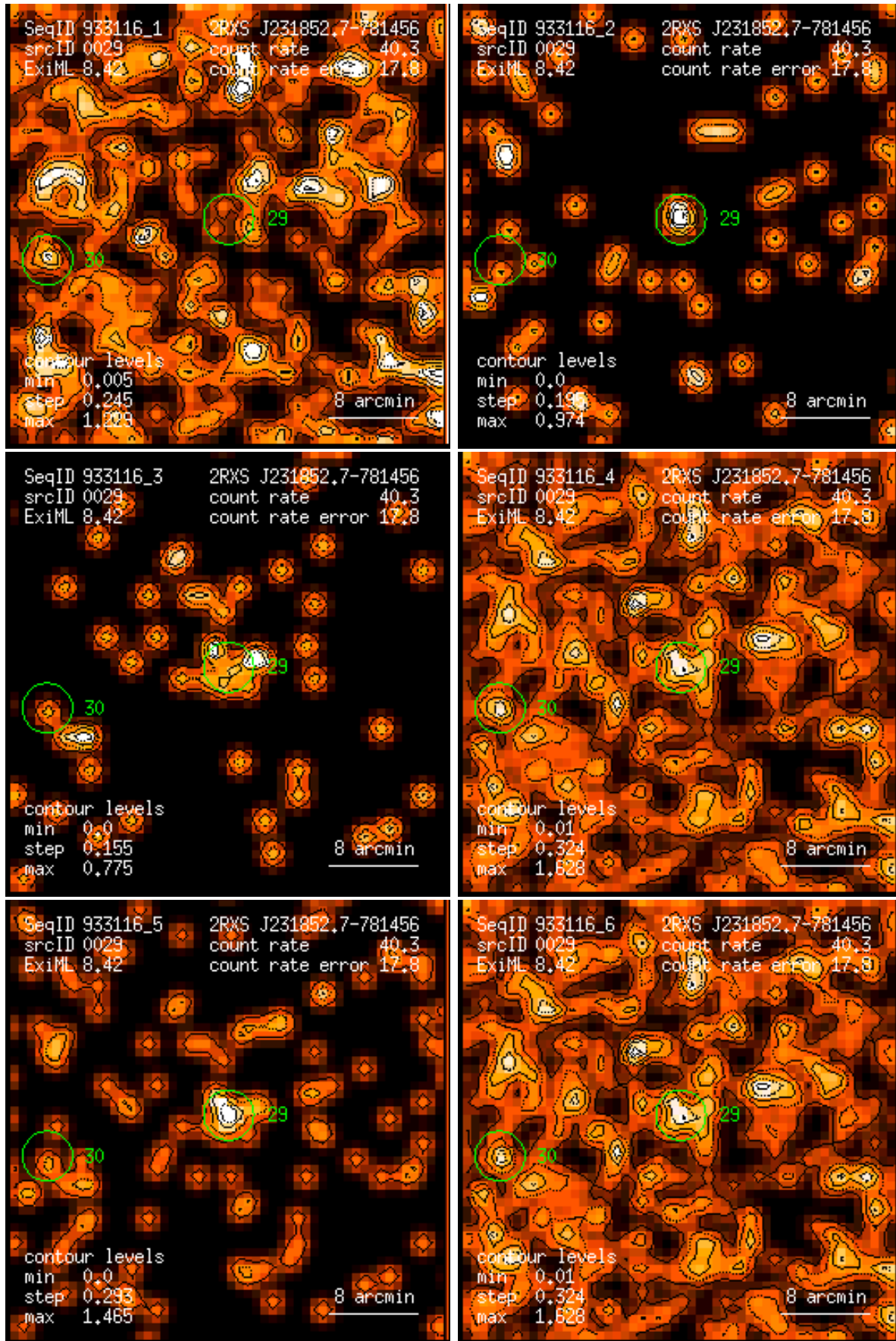
Figure 29: RASS 933116: detection 0029: band rate images, Gaussian filter: (1) PSPC channels 11 – 41, (2) 52 – 90, (3) 91 – 201, (4) 11 – 235, (5) 52 – 201, (6) 11 – 201. Broad band rates in counts/ks. Band rate contour levels in counts/ks/arcmin 2 .
