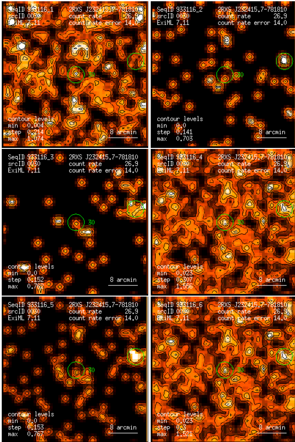
Figure 30: RASS 933116: detection 0030: band rate images, Gaussian filter: (1) PSPC channels 11 – 41, (2) 52 – 90, (3) 91 – 201, (4) 11 – 235, (5) 52 – 201, (6) 11 – 201. Broad band rates in counts/ks. Band rate contour levels in counts/ks/arcmin 2 .
