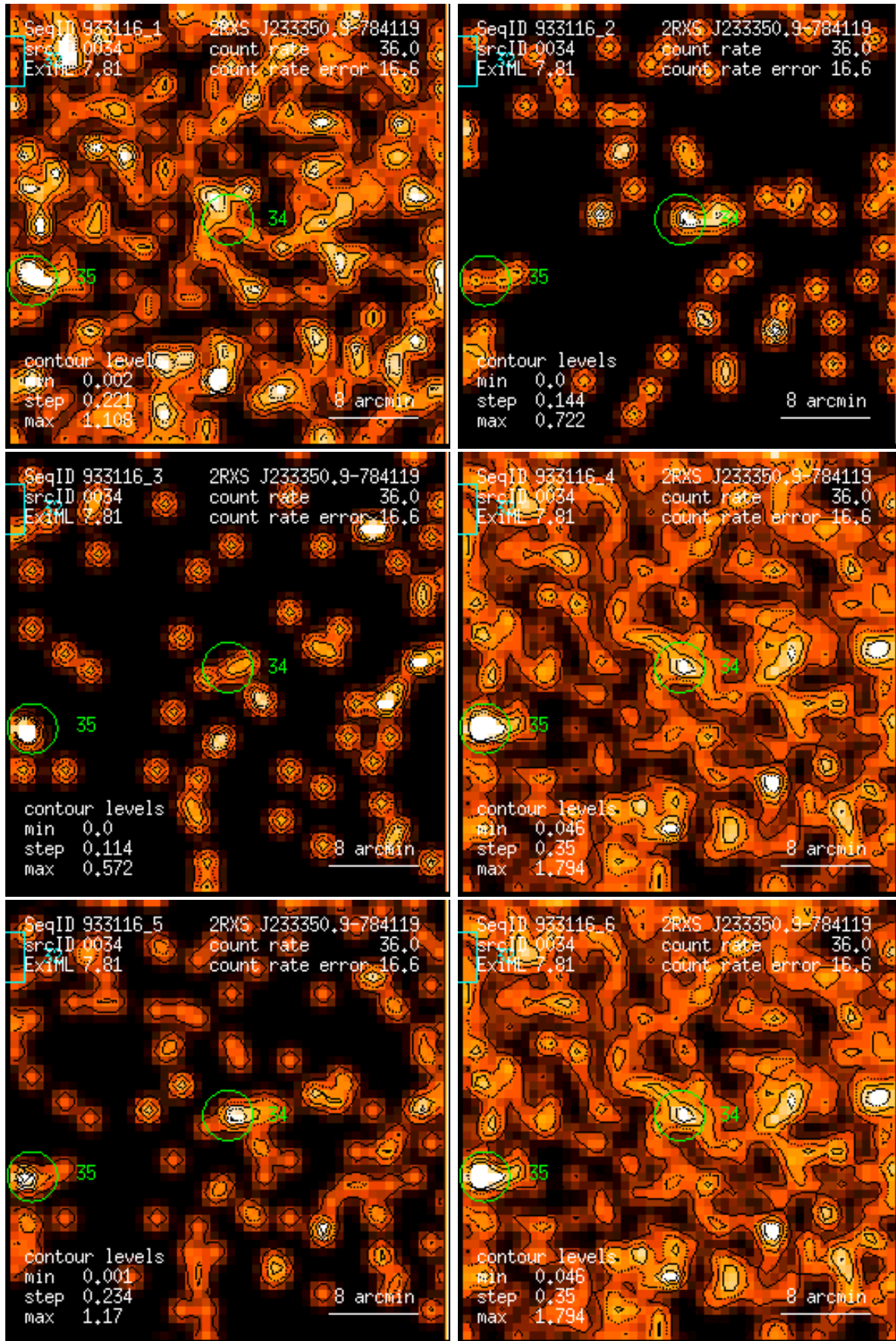
Figure 34: RASS 933116: detection 0034: band rate images, Gaussian filter: (1) PSPC channels 11 – 41, (2) 52 – 90, (3) 91 – 201, (4) 11 – 235, (5) 52 – 201, (6) 11 – 201. Broad band rates in counts/ks. Band rate contour levels in counts/ks/arcmin 2 .
