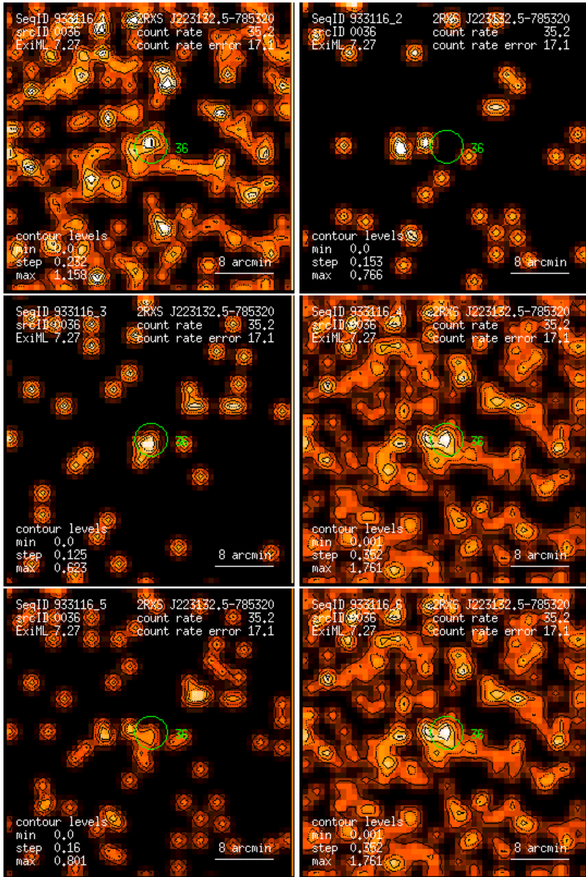
Figure 36: RASS 933116: detection 0036: band rate images, Gaussian filter: (1) PSPC channels 11 – 41, (2) 52 – 90, (3) 91 – 201, (4) 11 – 235, (5) 52 – 201, (6) 11 – 201. Broad band rates in counts/ks. Band rate contour levels in counts/ks/arcmin 2 .
