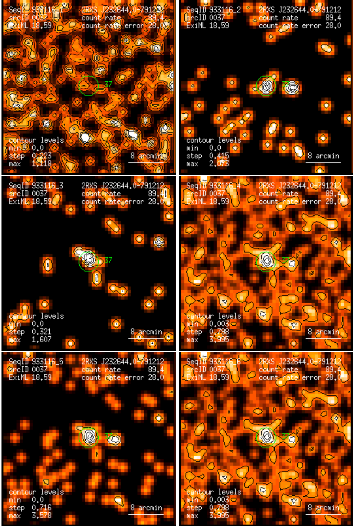
Figure 37: RASS 933116: detection 0037: band rate images, Gaussian filter: (1) PSPC channels 11 – 41, (2) 52 – 90, (3) 91 – 201, (4) 11 – 235, (5) 52 – 201, (6) 11 – 201. Broad band rates in counts/ks. Band rate contour levels in counts/ks/arcmin 2 .
