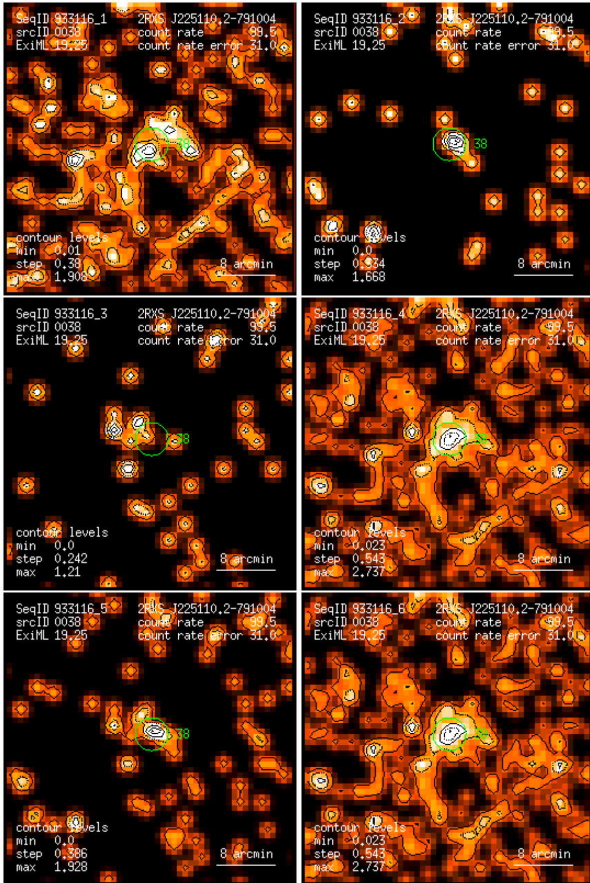
Figure 38: RASS 933116: detection 0038: band rate images, Gaussian filter: (1) PSPC channels 11 – 41, (2) 52 – 90, (3) 91 – 201, (4) 11 – 235, (5) 52 – 201, (6) 11 – 201. Broad band rates in counts/ks. Band rate contour levels in counts/ks/arcmin 2 .
