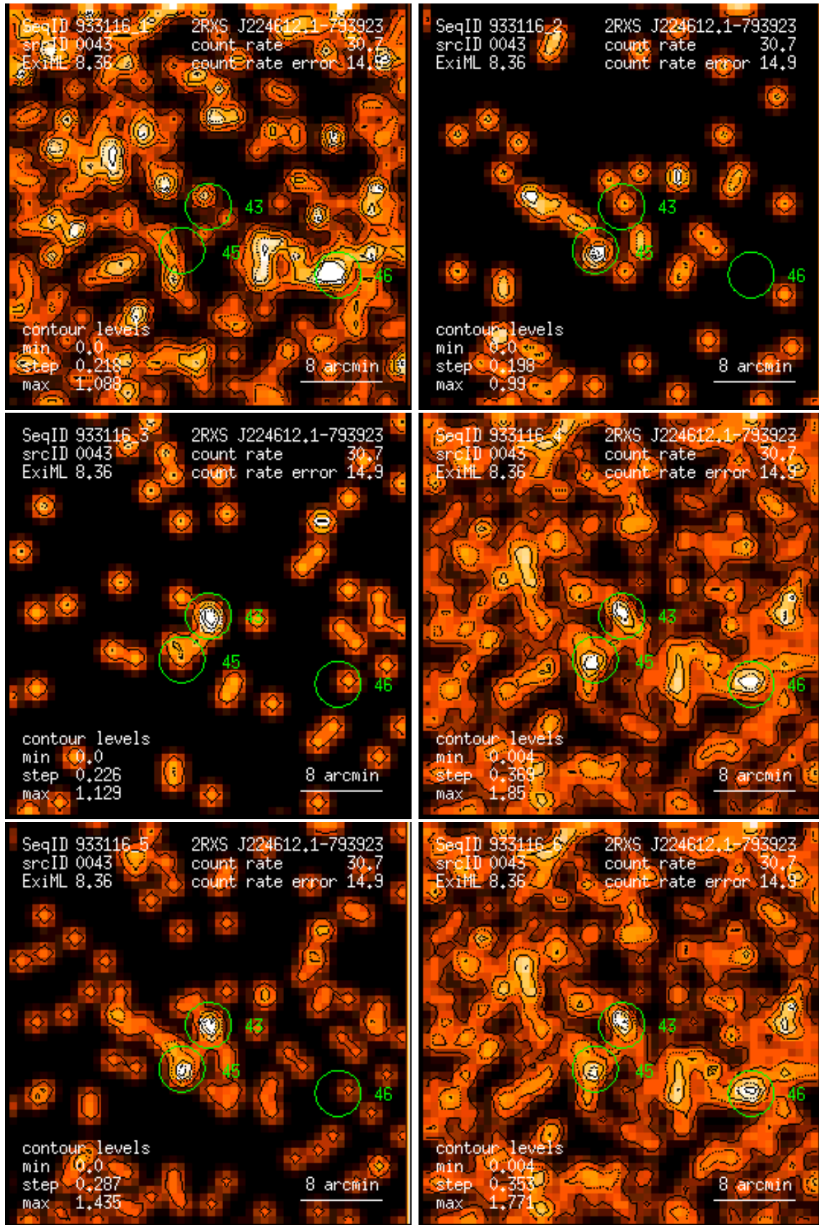
Figure 43: RASS 933116: detection 0043: band rate images, Gaussian filter: (1) PSPC channels 11 – 41, (2) 52 – 90, (3) 91 – 201, (4) 11 – 235, (5) 52 – 201, (6) 11 – 201. Broad band rates in counts/ks. Band rate contour levels in counts/ks/arcmin 2 .
