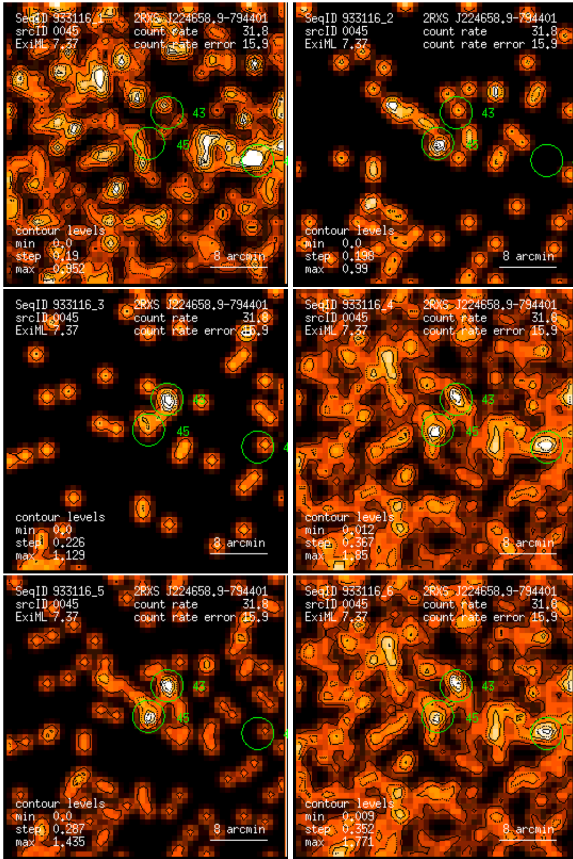
Figure 45: RASS 933116: detection 0045: band rate images, Gaussian filter: (1) PSPC channels 11 – 41, (2) 52 – 90, (3) 91 – 201, (4) 11 – 235, (5) 52 – 201, (6) 11 – 201. Broad band rates in counts/ks. Band rate contour levels in counts/ks/arcmin 2 .
