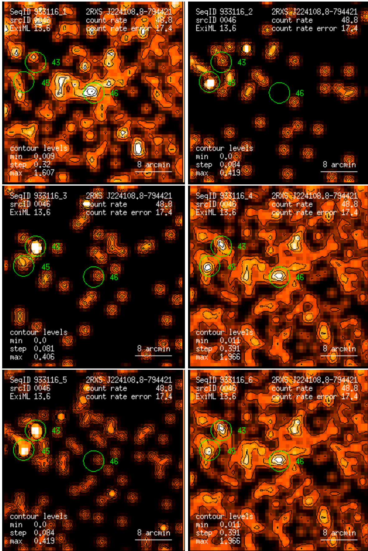
Figure 46: RASS 933116: detection 0046: band rate images, Gaussian filter: (1) PSPC channels 11 – 41, (2) 52 – 90, (3) 91 – 201, (4) 11 – 235, (5) 52 – 201, (6) 11 – 201. Broad band rates in counts/ks. Band rate contour levels in counts/ks/arcmin 2 .
