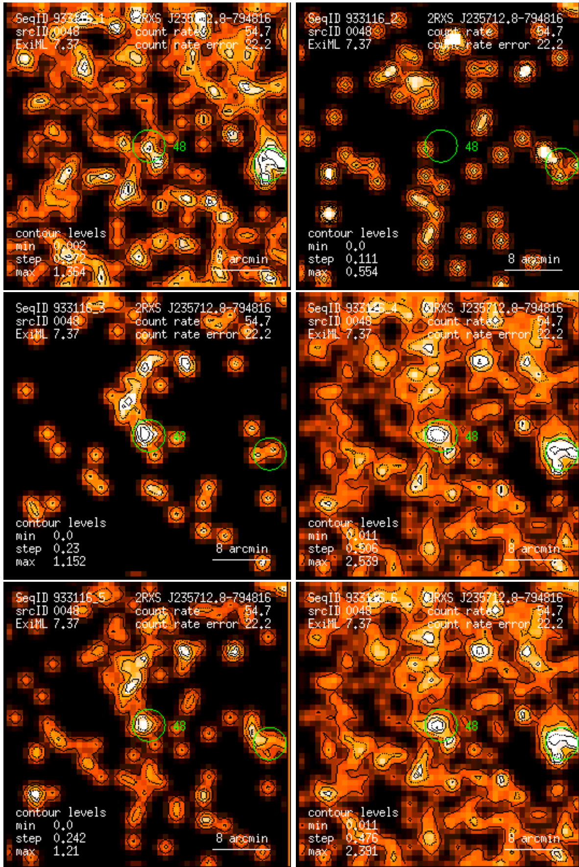
Figure 48: RASS 933116: detection 0048: band rate images, Gaussian filter: (1) PSPC channels 11 – 41, (2) 52 – 90, (3) 91 – 201, (4) 11 – 235, (5) 52 – 201, (6) 11 – 201. Broad band rates in counts/ks. Band rate contour levels in counts/ks/arcmin 2 .
