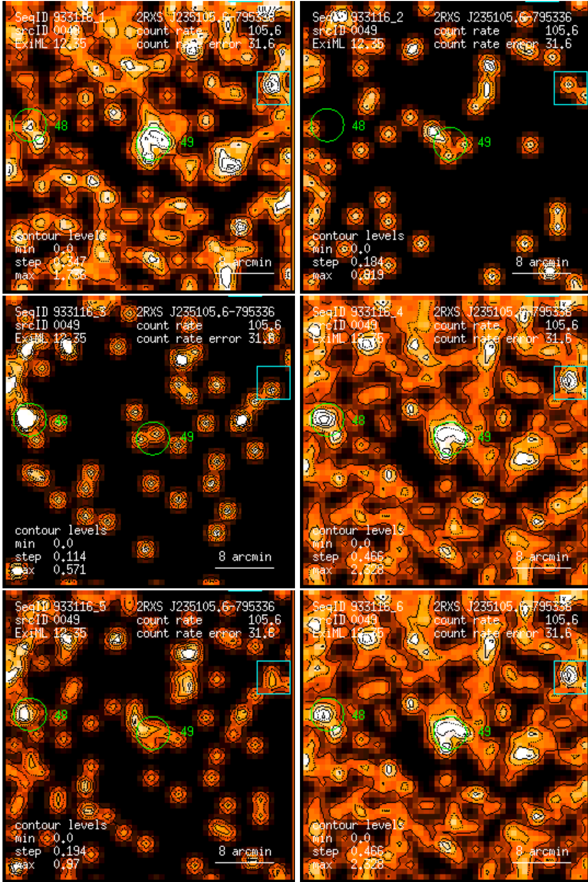
Figure 49: RASS 933116: detection 0049: band rate images, Gaussian filter: (1) PSPC channels 11 – 41, (2) 52 – 90, (3) 91 – 201, (4) 11 – 235, (5) 52 – 201, (6) 11 – 201. Broad band rates in counts/ks. Band rate contour levels in counts/ks/arcmin 2 .
