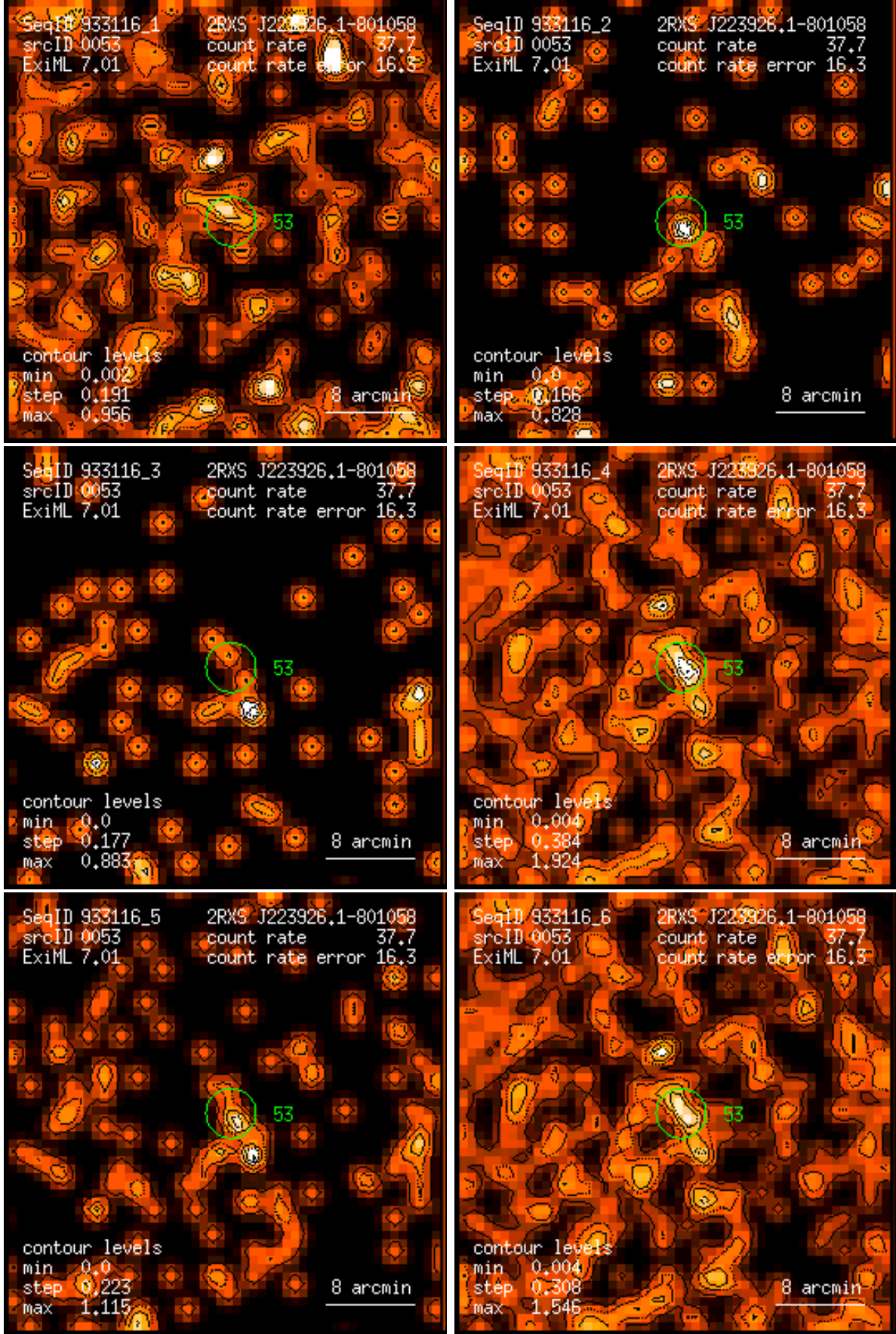
Figure 53: RASS 933116: detection 0053: band rate images, Gaussian filter: (1) PSPC channels 11 – 41, (2) 52 – 90, (3) 91 – 201, (4) 11 – 235, (5) 52 – 201, (6) 11 – 201. Broad band rates in counts/ks. Band rate contour levels in counts/ks/arcmin 2 .
